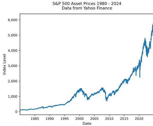
Figure 1.1: Raw Price Series
