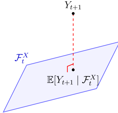
Figure 2.2: Conditional expectation as an orthogonal projection. The filtration \mathcal{F}_t^X defines a restricted information plane, while the conditional expectation is the projection of Y_{t+1} onto available information. Since Y_{t+1} may also depend on latent factors outside that plane, the residual reflects the limits of observable data.
