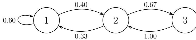
Figure 3.3: Topological representation of the empirically calibrated Markov chain.
