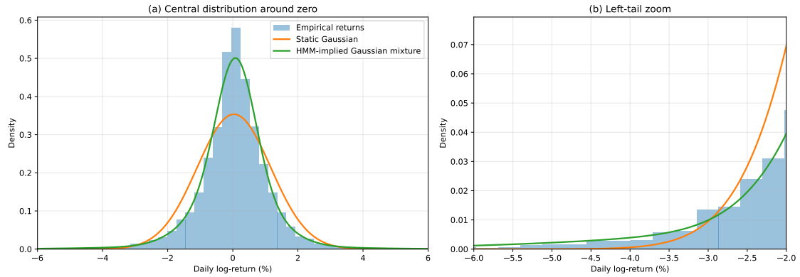
Figure 6.3: S&P 500 daily log-returns compared with a static Gaussian and the three-state Gaussian mixture implied by the HMM. (a) Full view shows the distribution around zero. (b) Zoomed view focuses on the left tail to highlight extreme returns.
