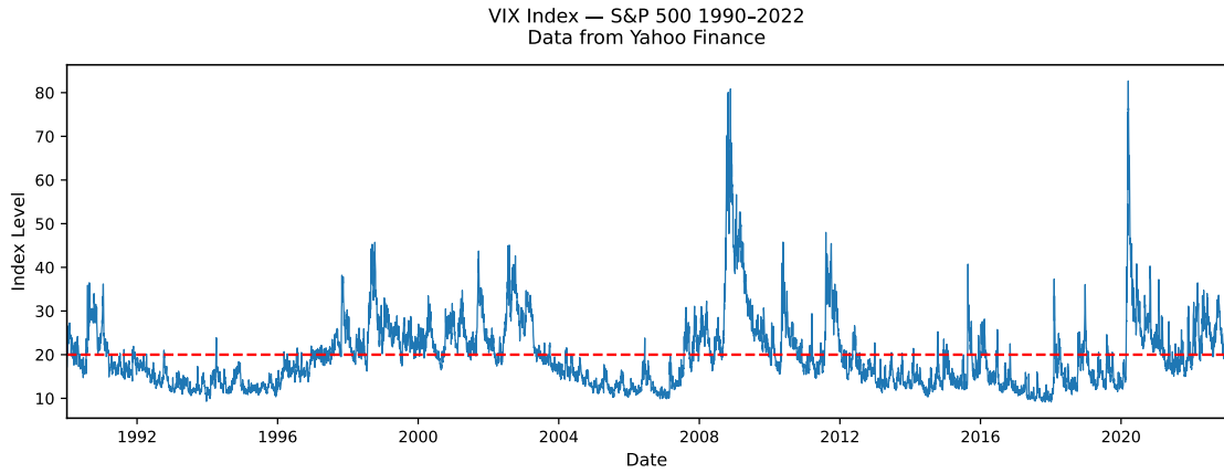
Figure 1.3: Path of the Volatility Index (VIX), a leading measure of market expectations of near-term volatility. The gap between the long-term average (red dashed line) and the realized level exposes the inadequacy of the constant variance assumption.
