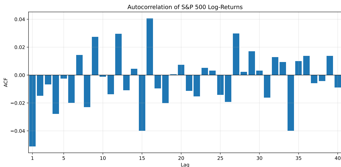
Figure 6.4: Autocorrelation function of S&P 500 daily log-returns.
