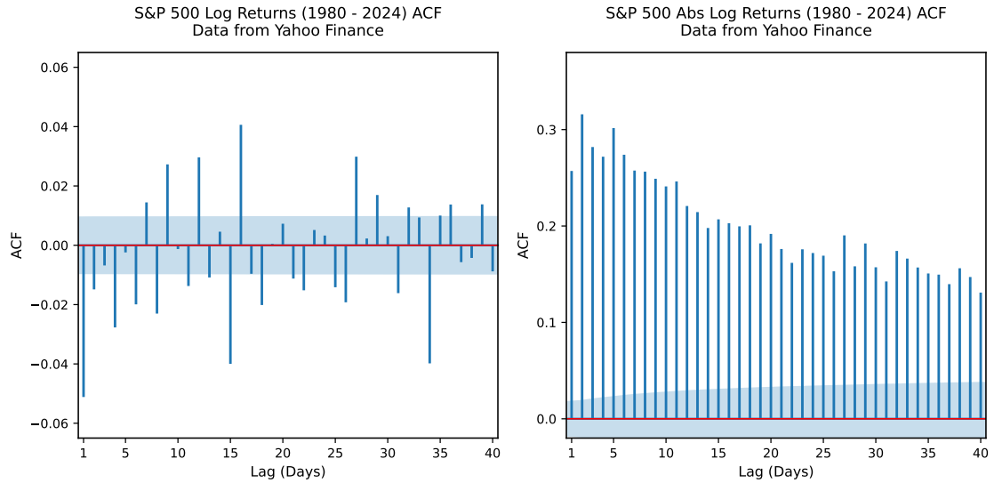
Figure 1.4: The left panel shows autocorrelation values close to zero, confirming the absence of linear dependence in raw returns. The right panel shows consistently positive values for absolute returns, revealing a strong persistence in magnitude.
