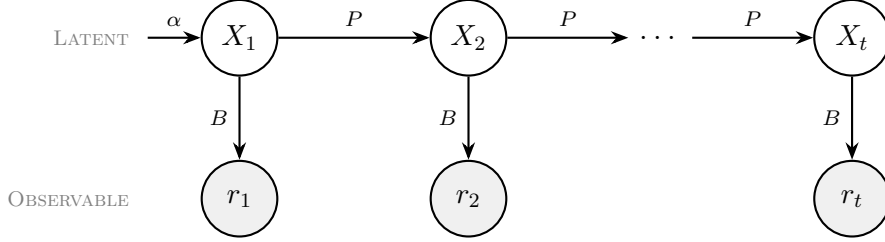
Figure 4.1: The distribution \alpha initializes the latent sequence, P propagates the hidden transitions, and B determines the density generating the return r_t .
