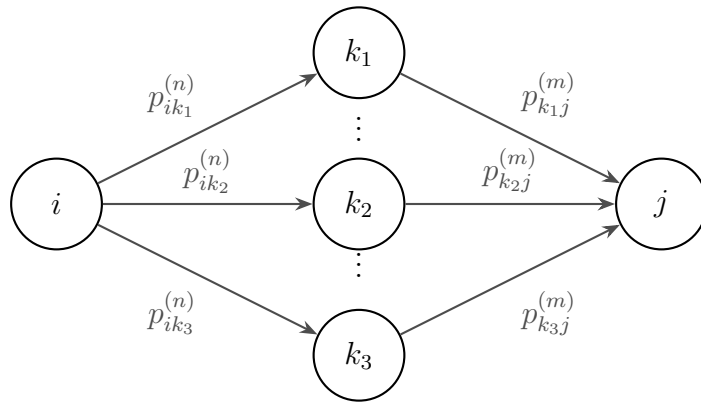
Figure 3.2: The (n + m) -step transition probability is obtained by marginalizing over the intermediate state at time n , summing over k \in \mathcal{S} the product of the n -step and m -step transition probabilities, a factorization justified by the Markov property.
