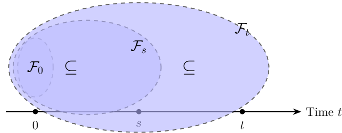
Figure 2.1: Representation of a filtration \mathbb{F} = \{\mathcal{F}_t\}_{t \geq 0} . As time progresses along the horizontal axis, the \sigma -algebras expand ( \mathcal{F}_0 \subseteq \mathcal{F}_s \subseteq \mathcal{F}_t ), illustrating the accumulation of historical data and the set of events with known outcomes to the market observer.
