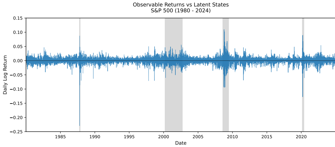
Figure 2.3: The illustration of partial information highlights the distinction between observable data and latent market dynamics. The solid line represents the logarithmic returns, while the shaded regions reflect unobserved states associated with periods of high volatility, capturing the market turbulence not visible in the return series.
