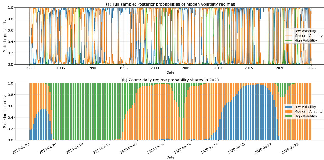
Figure 6.2: Posterior probabilities of the hidden volatility regimes. (a) The full sample shows the evolution of regime probabilities over the time window. (b) The zoomed 2020 market-stress period represents each trading day as a stacked bar.
