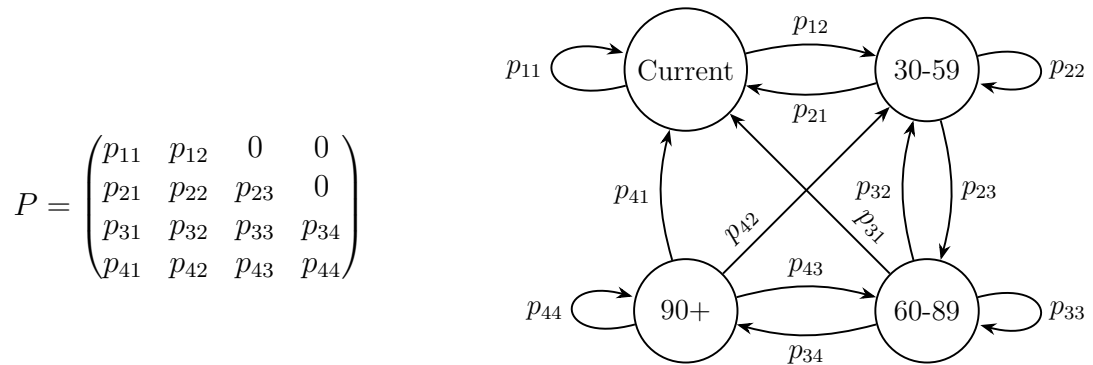
Figure 3.1: Algebraic and topological representation of local conditional dependence.
