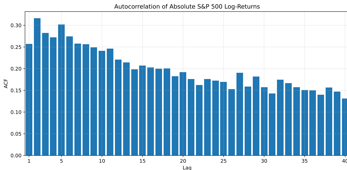
Figure 6.5: Autocorrelation function of S&P 500 absolute daily log-returns.
