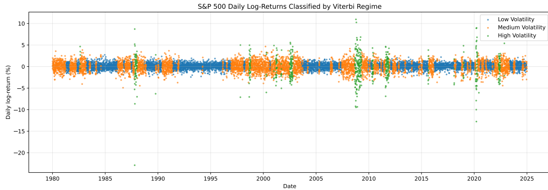
Figure 6.1: S&P 500 daily log-returns classified by Viterbi volatility regime.
