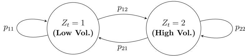
Figure 2.4: The nodes represent the latent market regimes: low volatility and high volatility, while the directed edges indicate the transition probabilities p_{ij} . This diagram formalizes the dynamics of switching between distinct structural phases.
