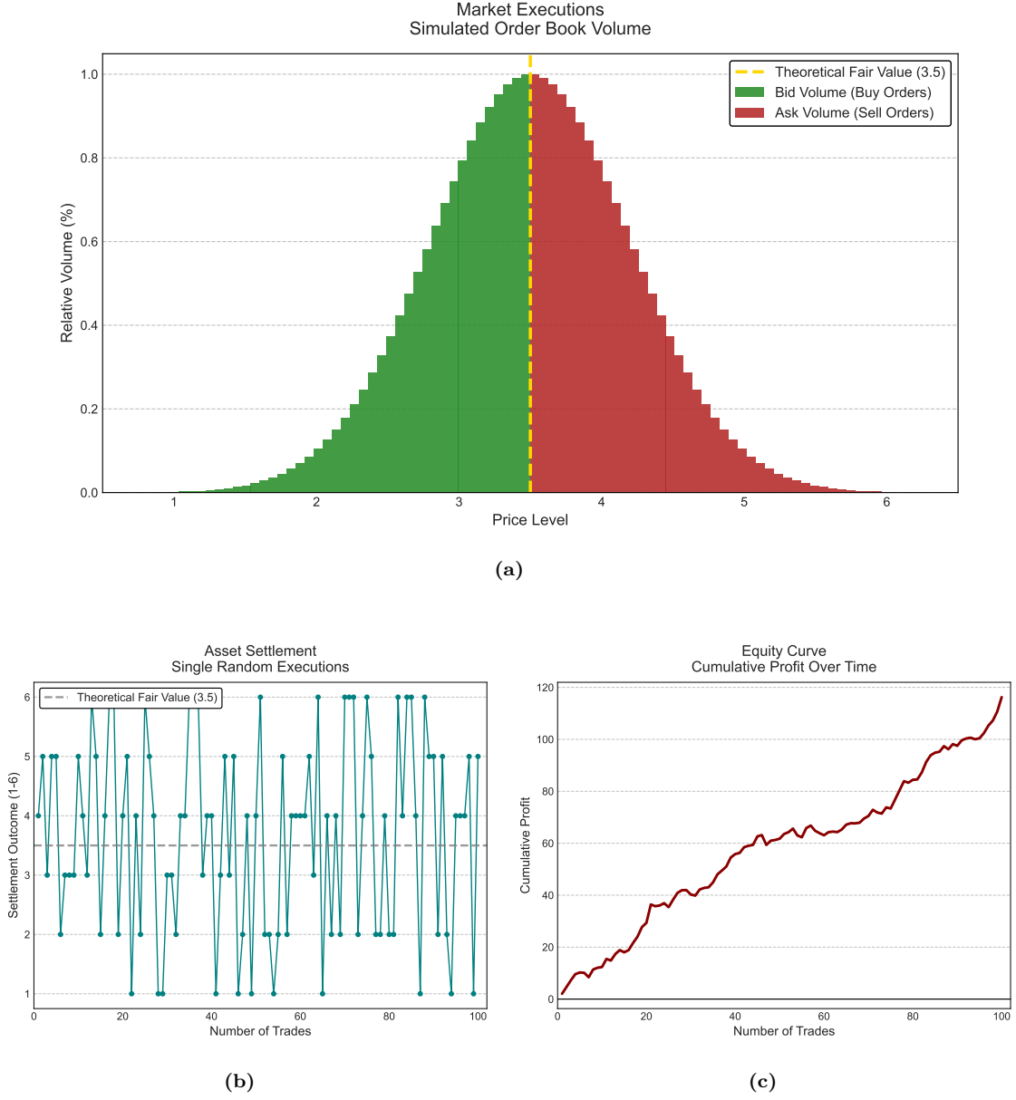
Figure 1.6: Simulation of a market maker in a strictly stationary environment. (a) Knowing the theoretical fair value (3.5), the market maker places bid volumes below this level and ask volumes above it, concentrating it around the center of the distribution. (b) The settlement value of each trade, simulated as a die roll, is random and uniformly distributed, illustrating short-term unpredictability. (c) Despite the randomness of individual settlements, the equity curve rises. Thus, in this stationary setting, the LLN explains the stabilization of average outcomes.
