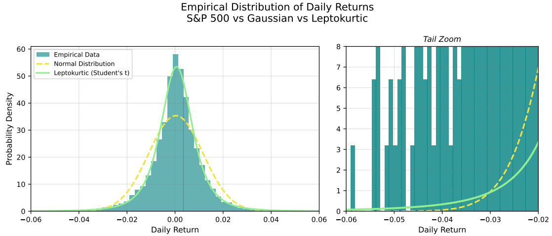
Figure 1.5: The comparison between empirical log returns, the Normal distribution and the fitted Student's t distribution ( \nu = 3 degrees of freedom, estimated from data using Python) shows how the Gaussian curve assigns insufficient probability mass to tails, thereby underestimating the likelihood of extreme events like the 1987 crash.
