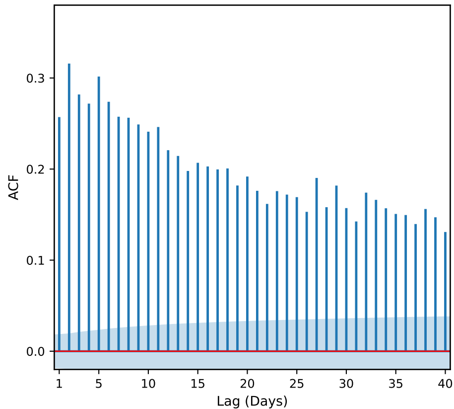
S&P 500 Abs Log Returns (1980 - 2024) ACF Data from Yahoo Finance
