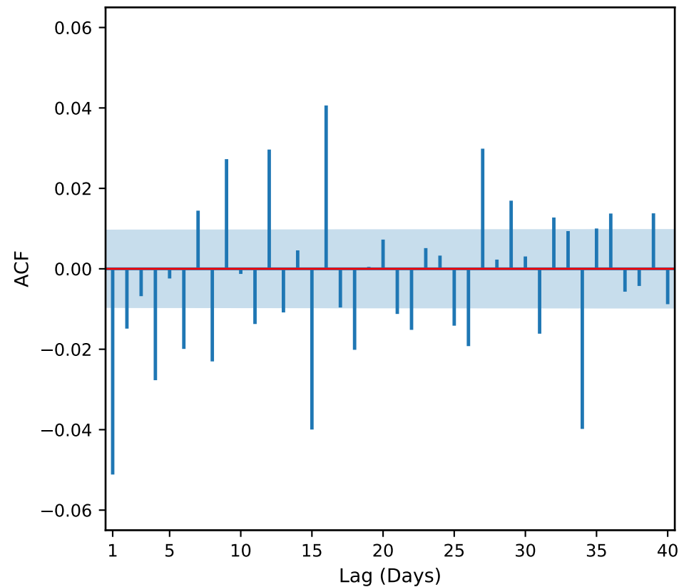
S&P 500 Log Returns (1980 - 2024) ACF Data from Yahoo Finance
