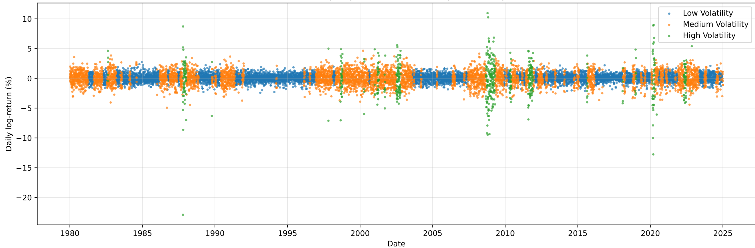
S&P 500 Daily Log-Returns Classified by Viterbi Regime
