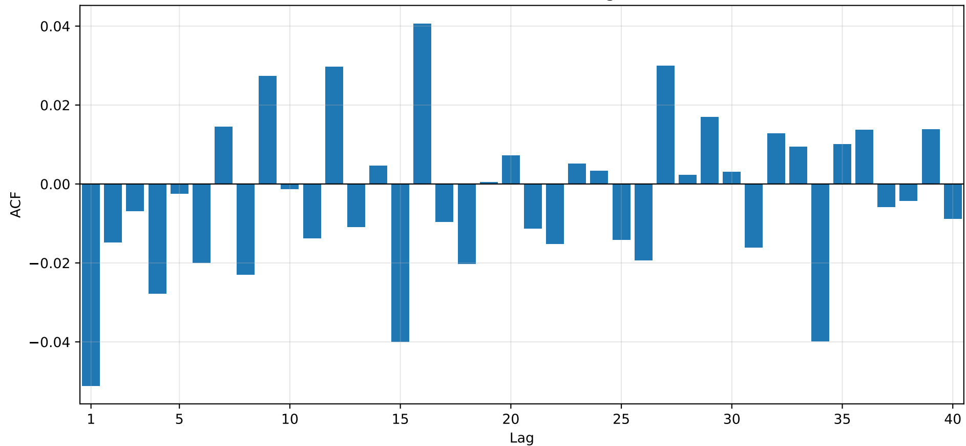
Autocorrelation of S&P 500 Log-Returns
