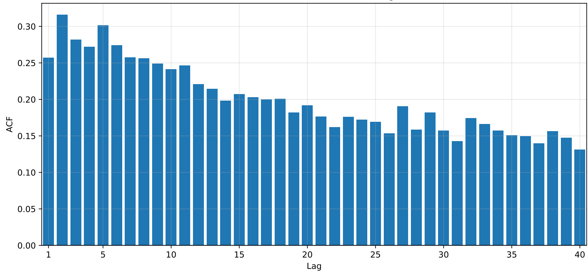
Autocorrelation of Absolute S&P 500 Log-Returns
