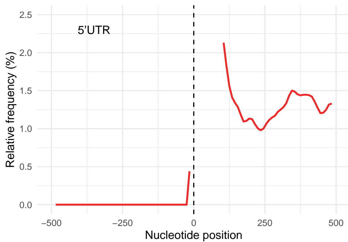
Start codon
