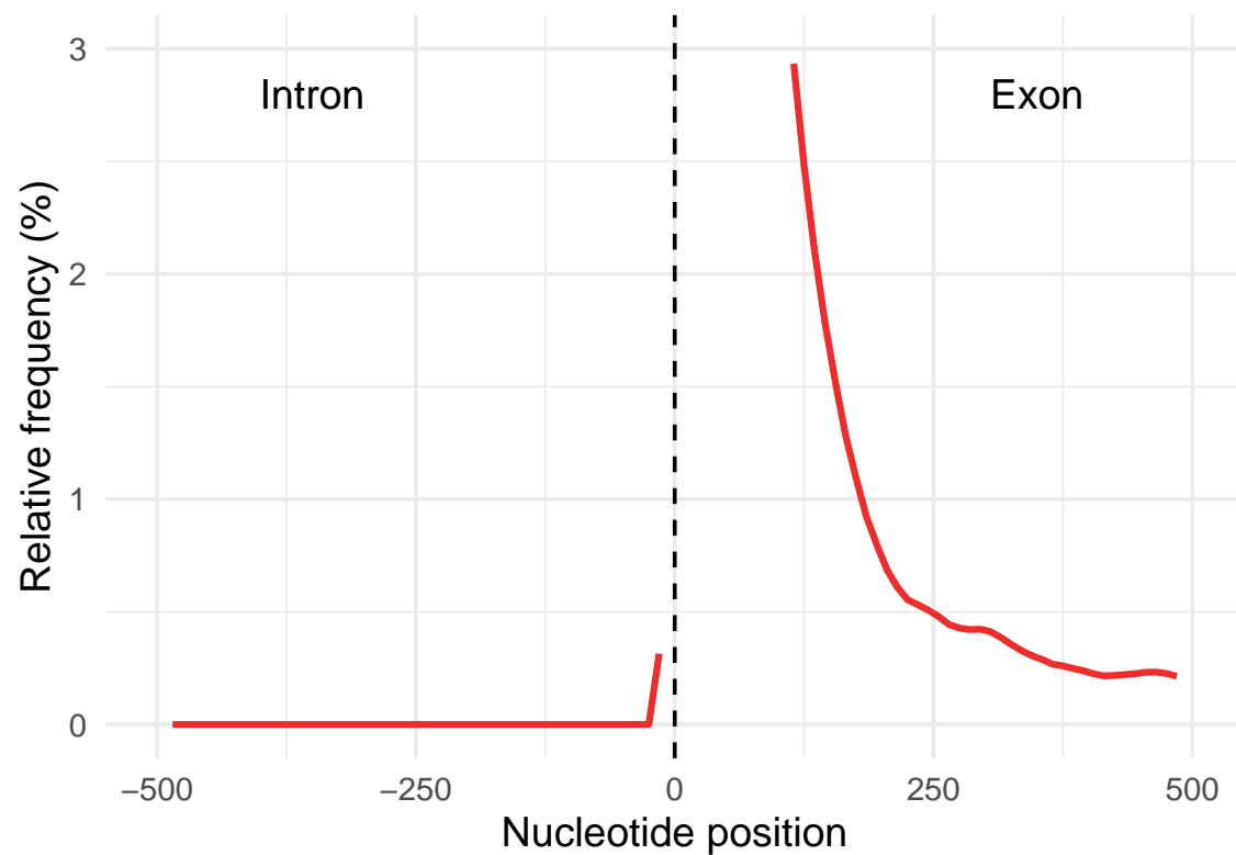
Stop codon
