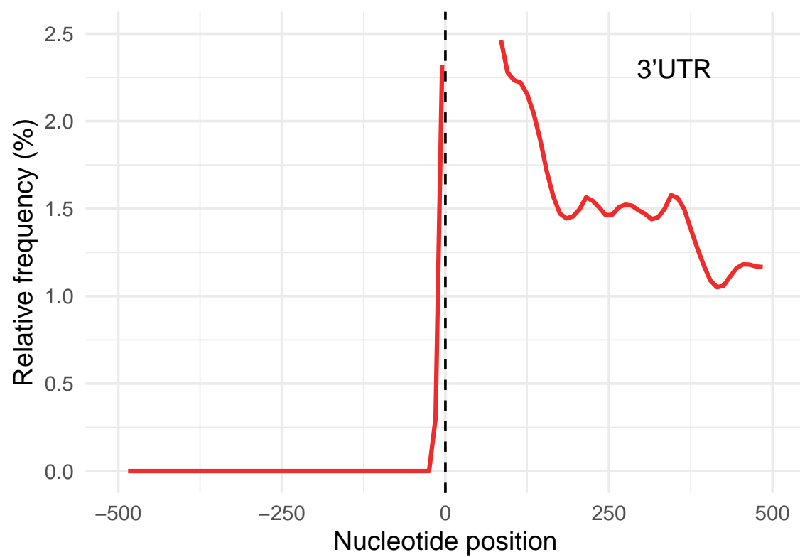
Stop codon
