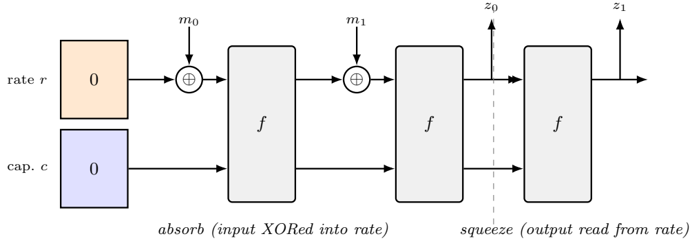
Figure 6.1: The duplex sponge. In the absorb phase each input block m_i is XORed into the rate and the state is passed through the permutation f ; in the squeeze phase output blocks z_i are read from the rate, applying f again between reads. The capacity is never read from or written to directly, which is what carries the security of the construction.
