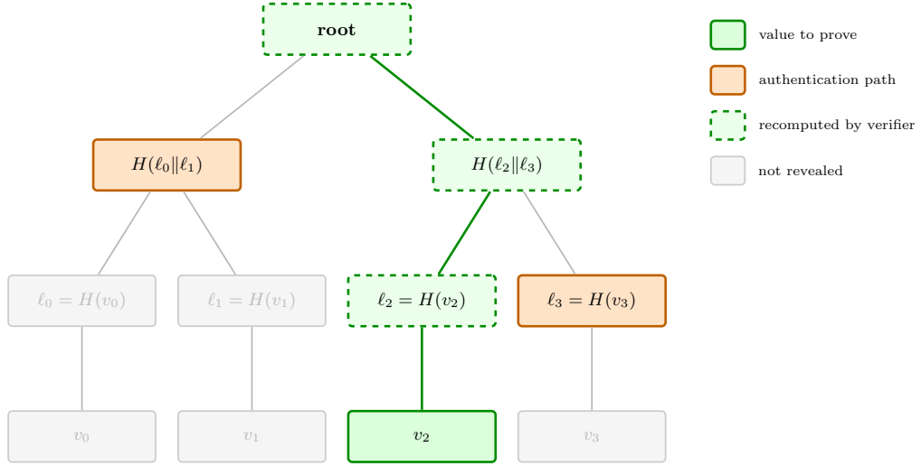
Figure 3.1: Verification of v_2 in a four-leaf Merkle tree. The prover reveals the authentication path (the two siblings \ell_3 and H(\ell_0||\ell_1) , in orange); the verifier recomputes the dashed nodes from v_2 up to the root and compares the result with the committed root. The greyed-out nodes are never revealed.
