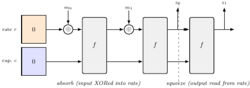
Figure 5.1: The duplex sponge. In the absorb phase each input block m_i is XORed into the rate and the state is passed through the permutation f ; in the squeeze phase output blocks z_i are read from the rate, applying f again between reads. The capacity is never read from or written to directly, which is what carries the security of the construction.
