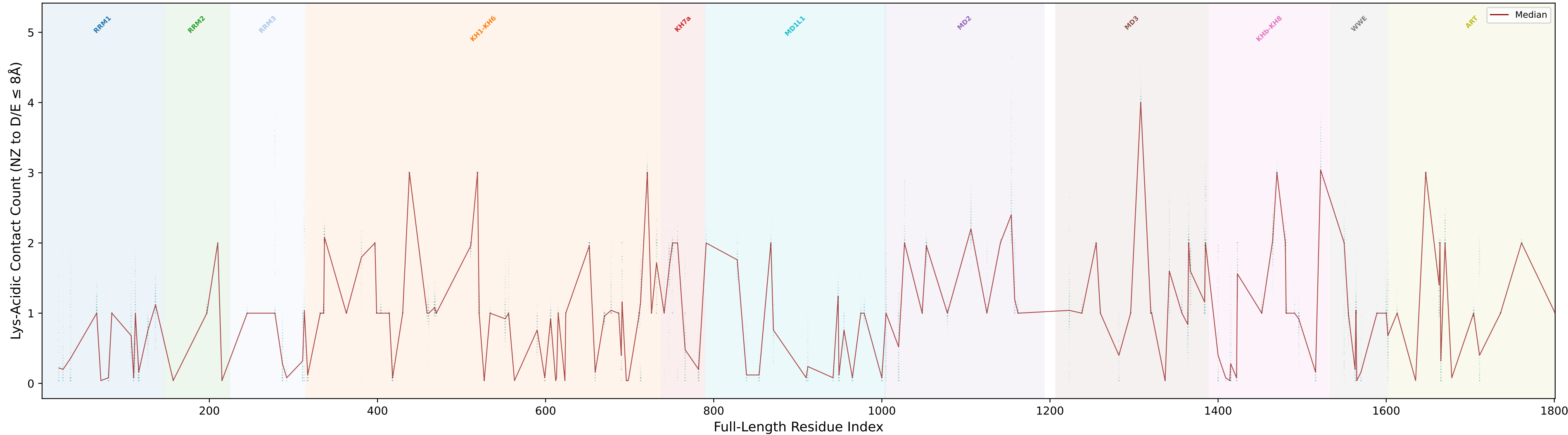
Per-Lysine Acidic Contact Count Across Constructs
