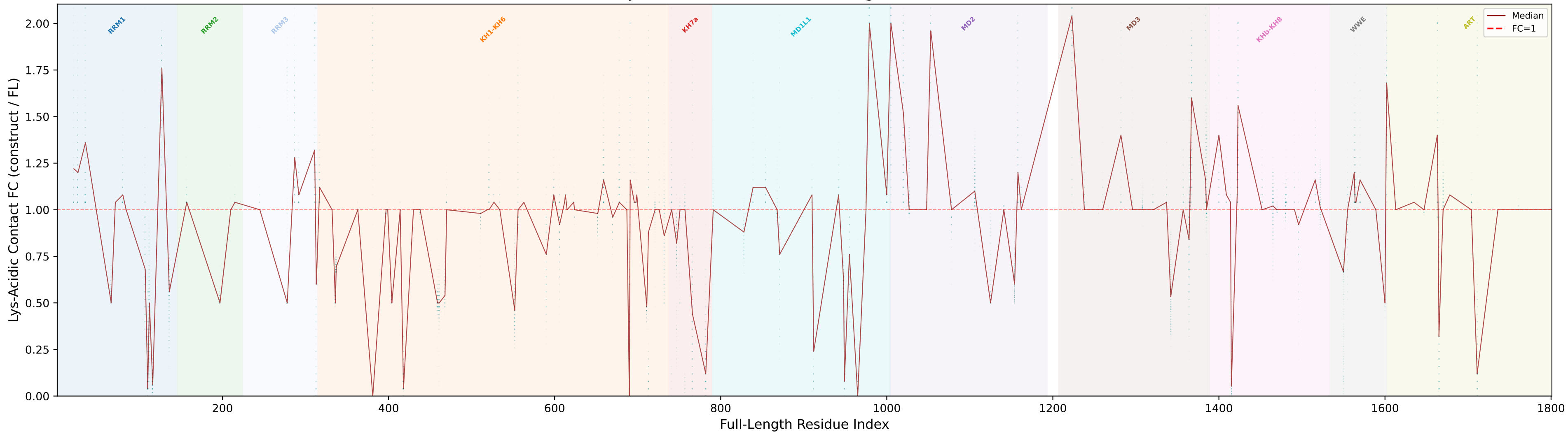
Per-Lysine Acidic Contact Fold Change (NZ to D/E \leq 8\text{\AA} )
