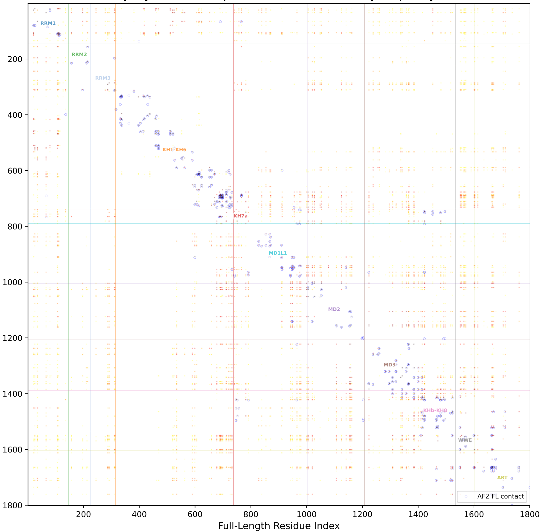
Lys-Lys Contact Map (NZ-NZ \leq 16\text{\AA} , colored by frequency)
