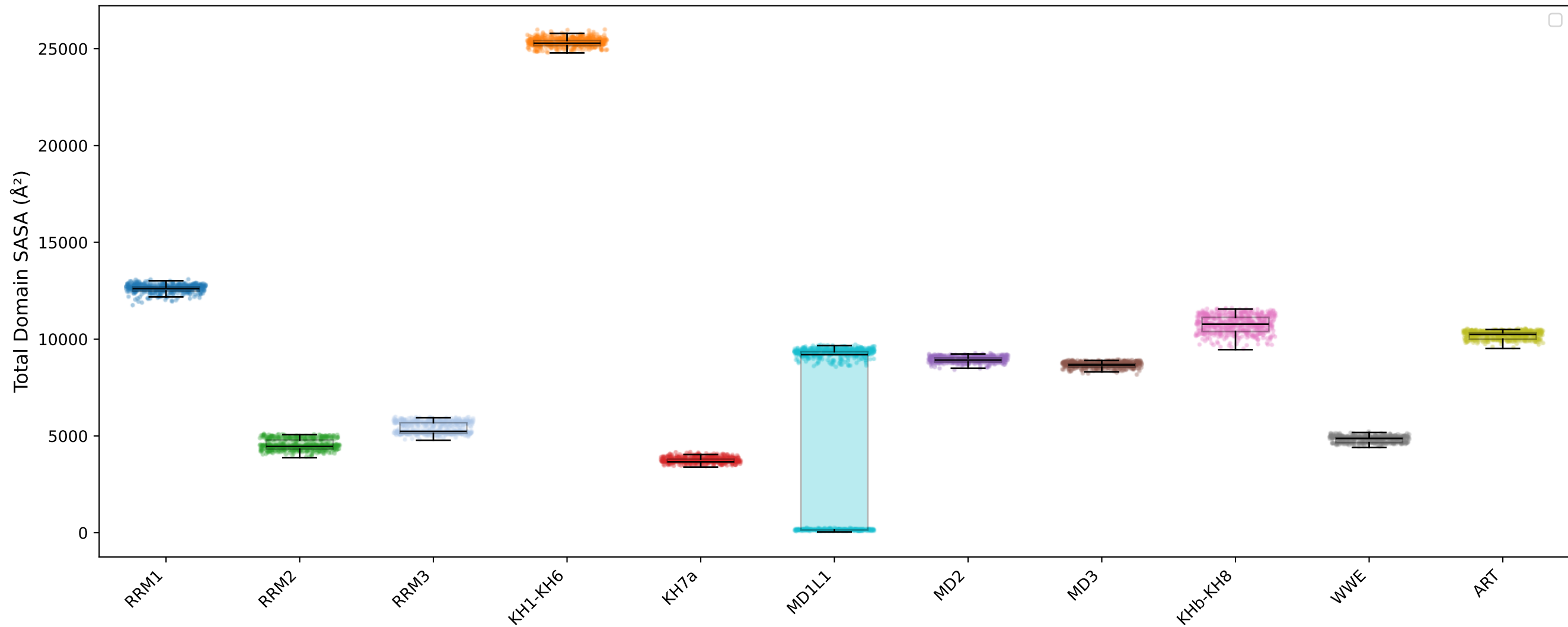
Per-Domain Total SASA Across Domain Deletion Constructs
