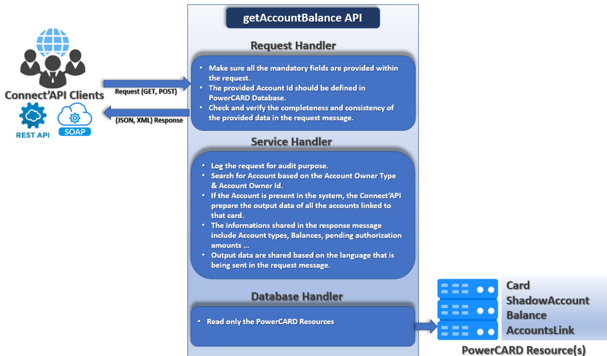
Figure 21: getAccountBalance process
