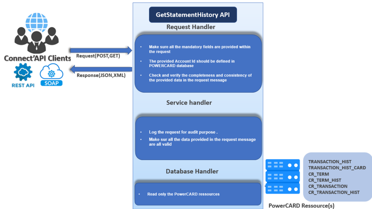
Figure 37: GetStatementHistory process
