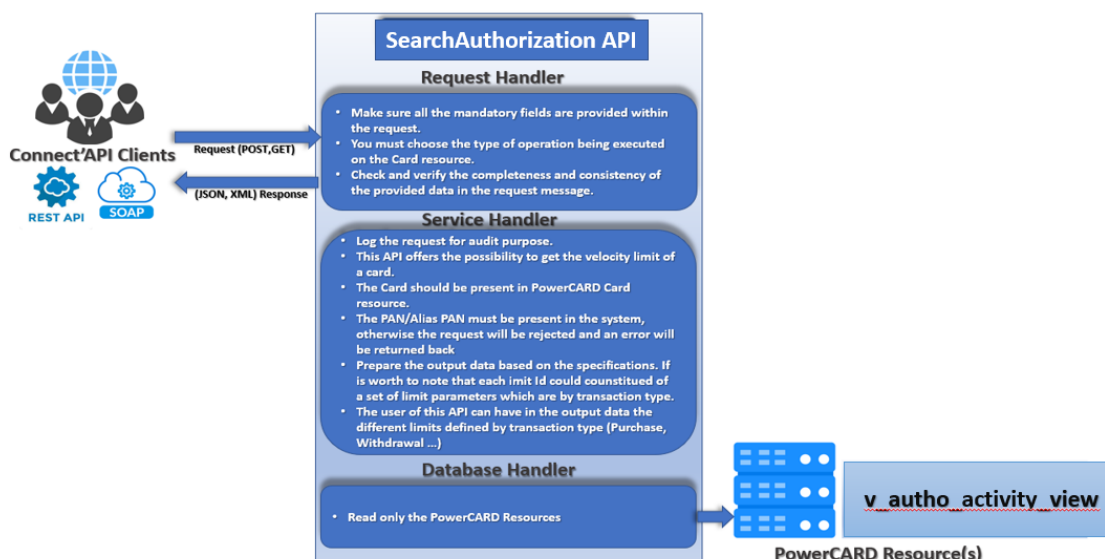
Figure 33: searchAuthorization process
