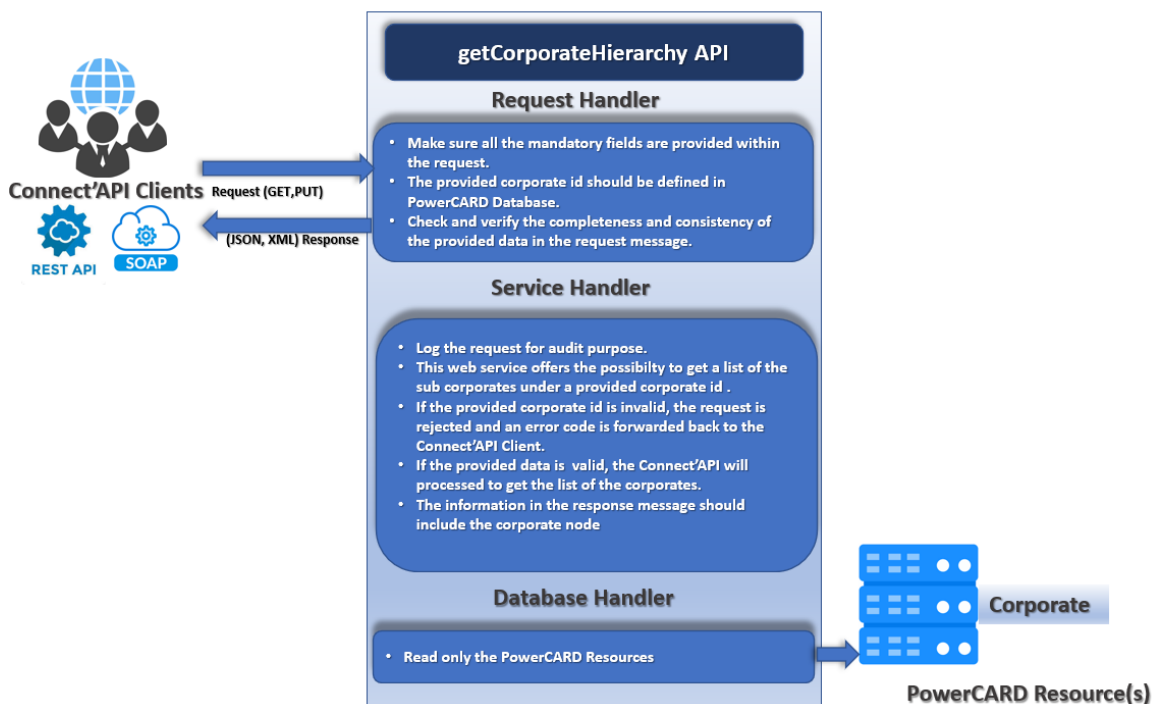
Figure 60: getCorporateHierarchy process
