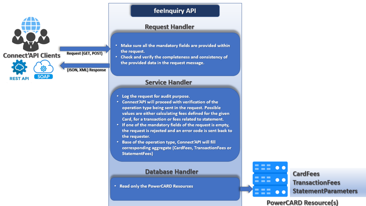
Figure 13: feelInquiry process
