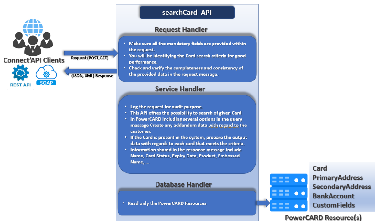
Figure 4: searchCard process
