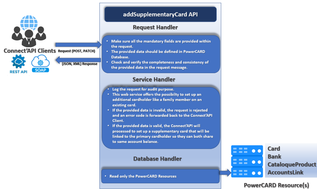
Figure 55: addSupplementaryCard process
