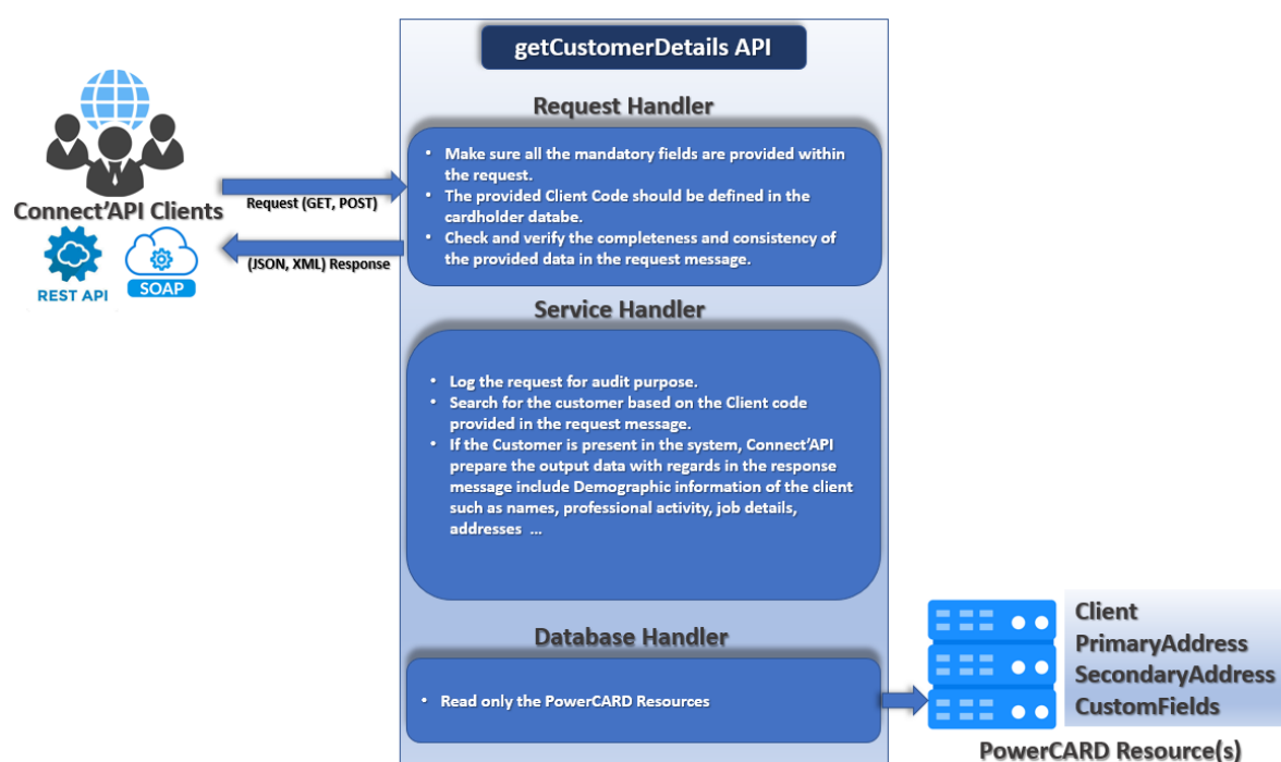
Figure 11: getCustomerDetails process
