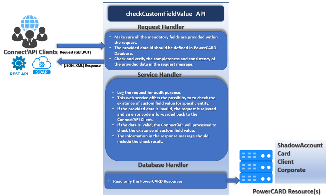
Figure 48: checkCustomFieldValue process
