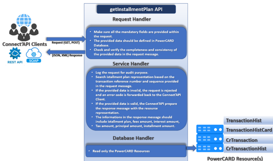
Figure 45: getInstallmentPlan process
