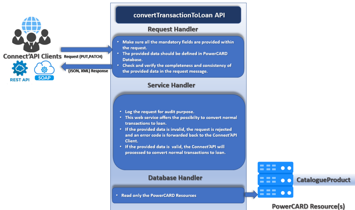
Figure 57: convertTransactionToLoan process
