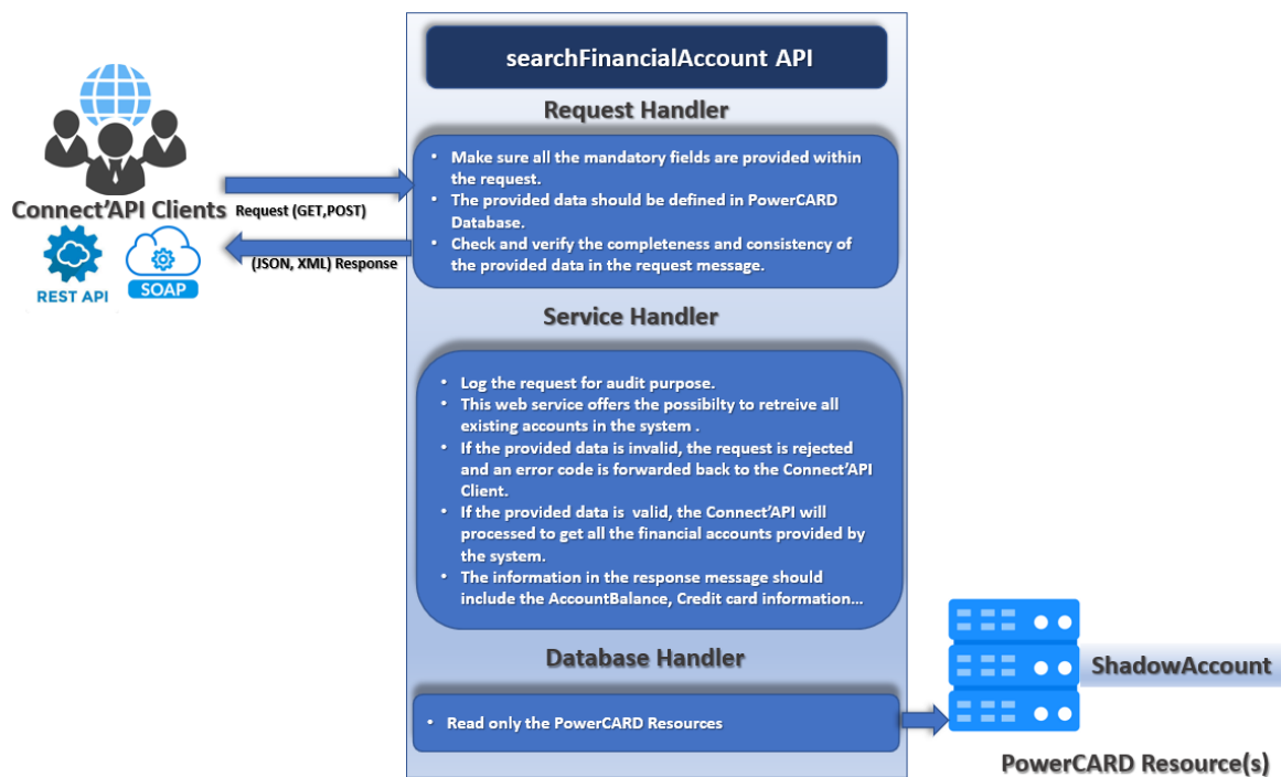
Figure 54: searchFinancialAccount process
