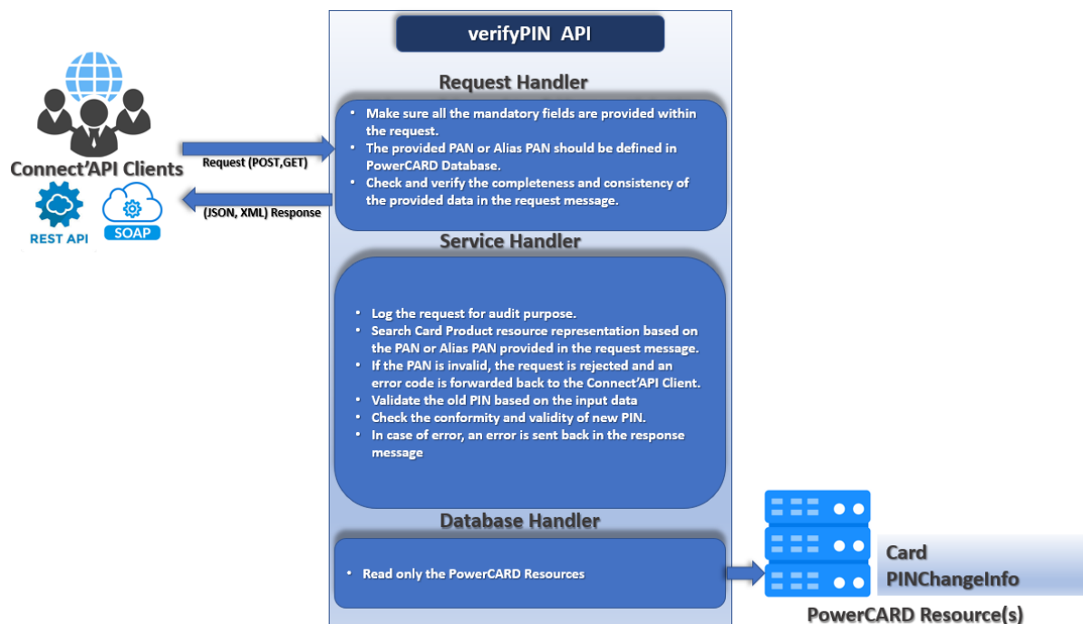
Figure 29: verifyPIN process
