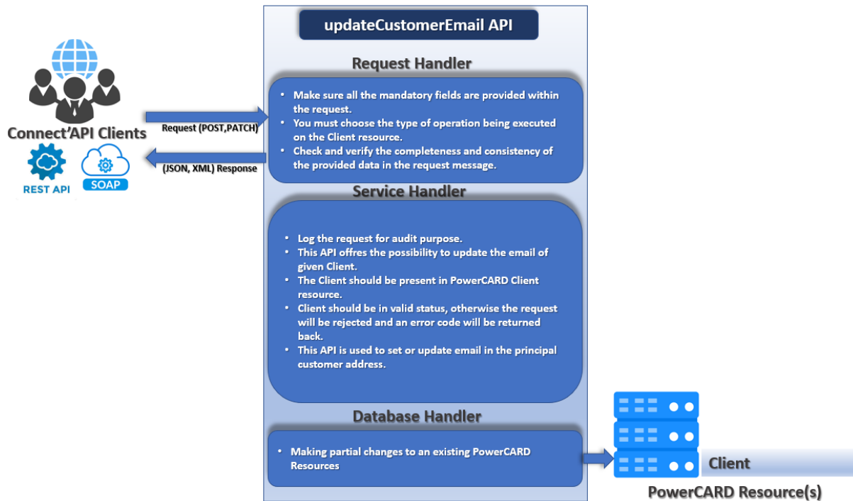
Figure 15: updateCustomerEmail process
