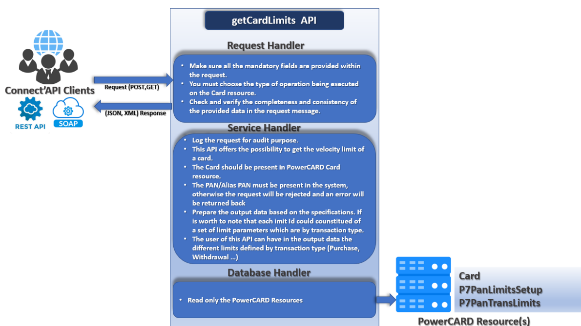
Figure 25: getCardLimitsprocess
