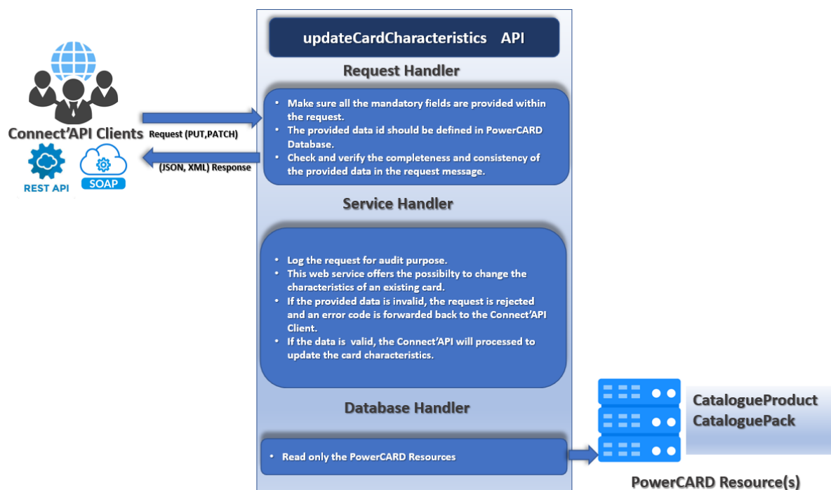
Figure 67: updateCardCharacteristics process
