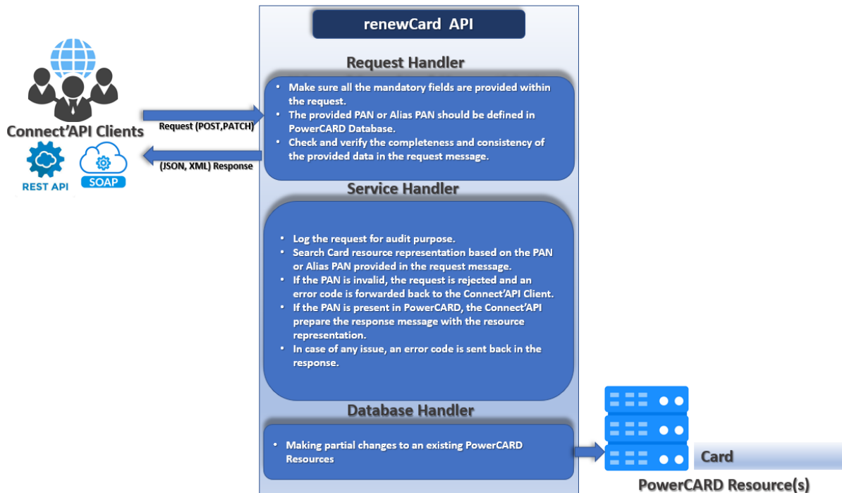
Figure 6: renewCard process
