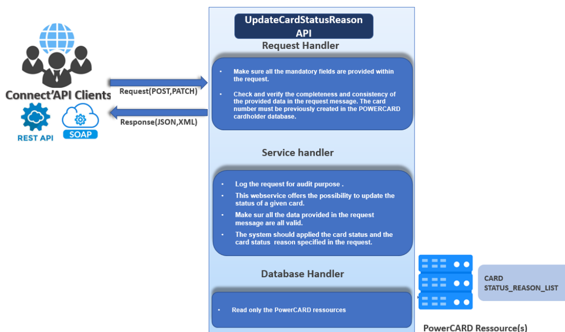
Figure 63: updateCardStatusReason process
