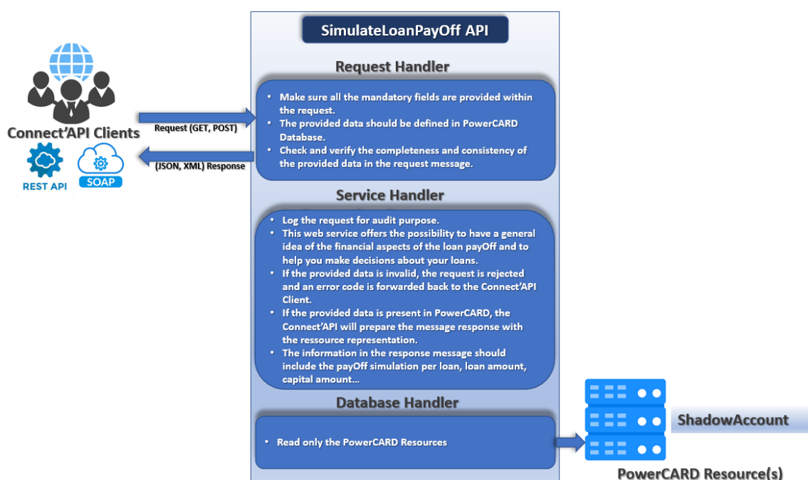
Figure 81: SimulateLoanPayOff process
