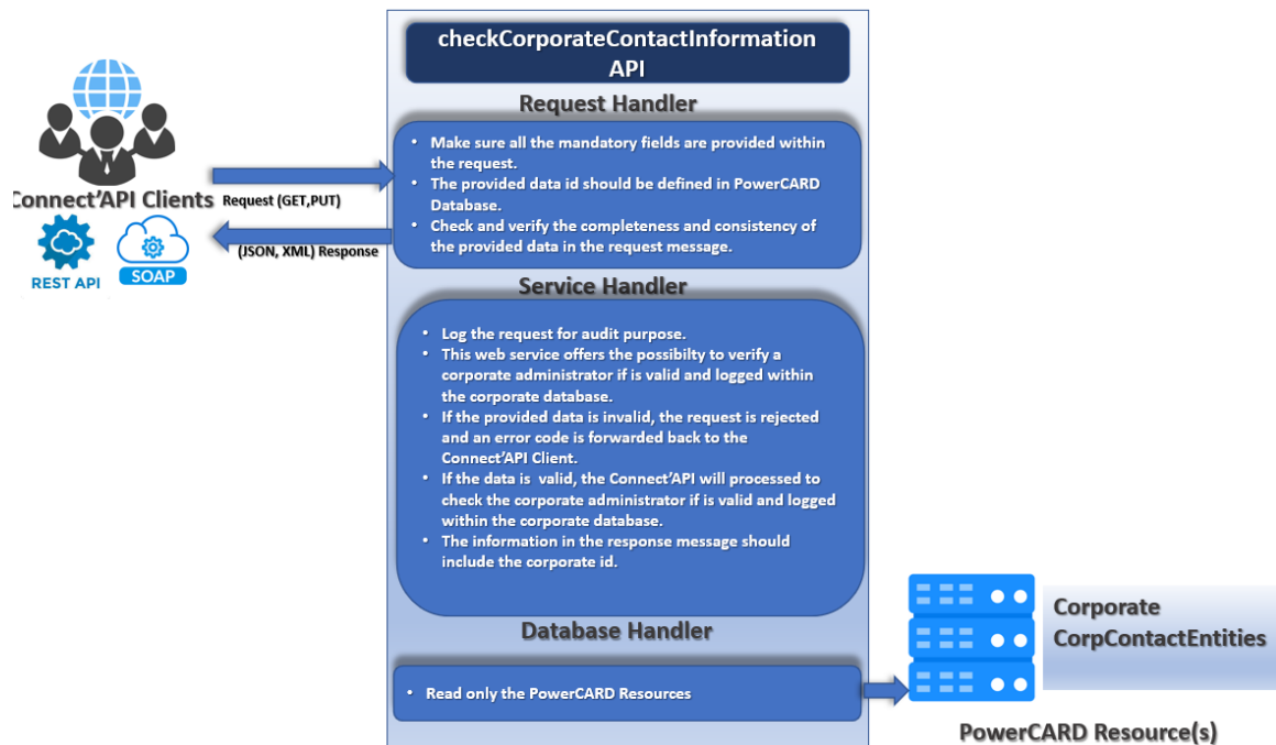
Figure 42: checkCorporateContactInformation
