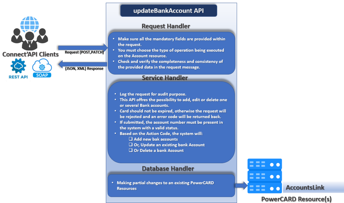
Figure 17: updateBankAccount process
