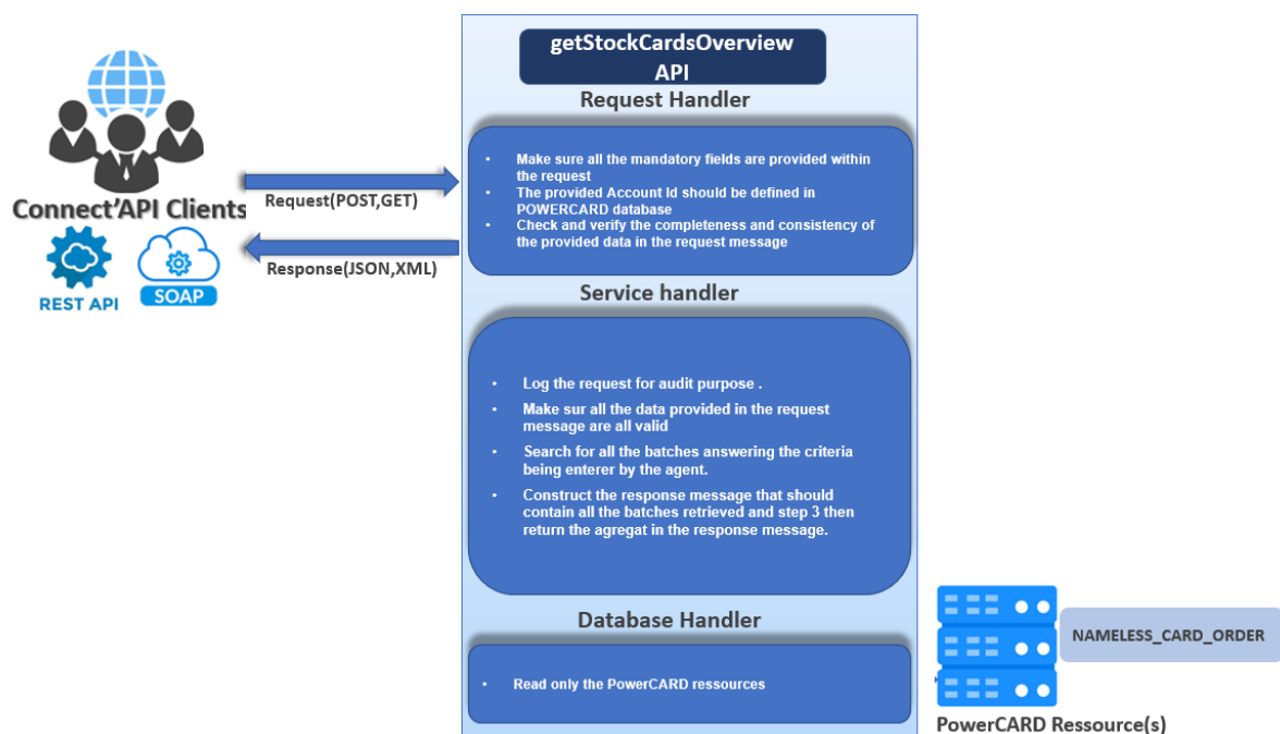
Figure 36: GetStockCardsOverview process
