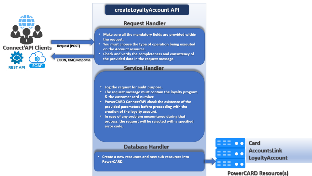
Figure 19: createLoyaltyAccount process
