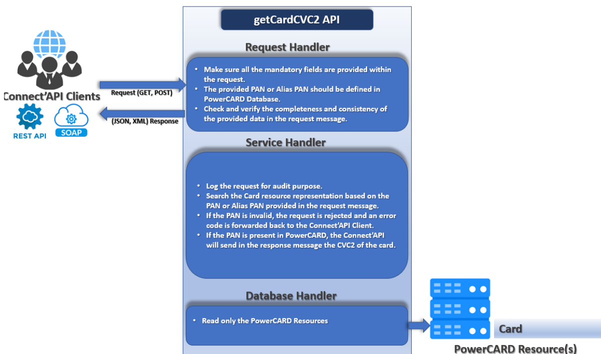
Figure 10: getCardCVC2 process
