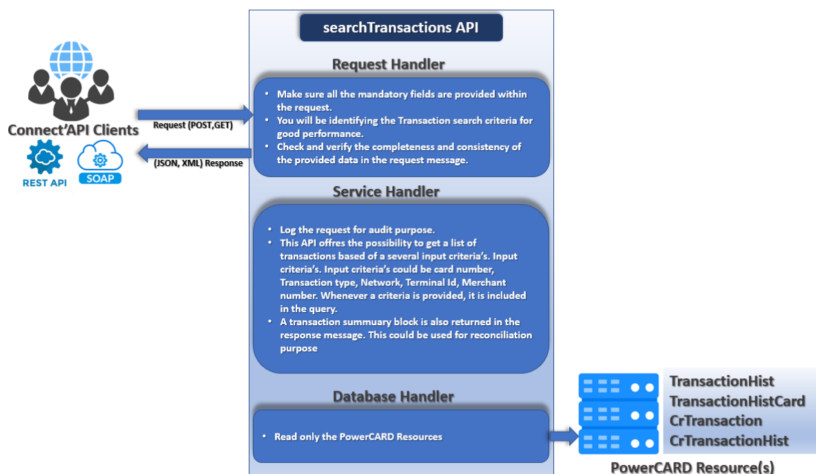
Figure 16: searchTransactions process
