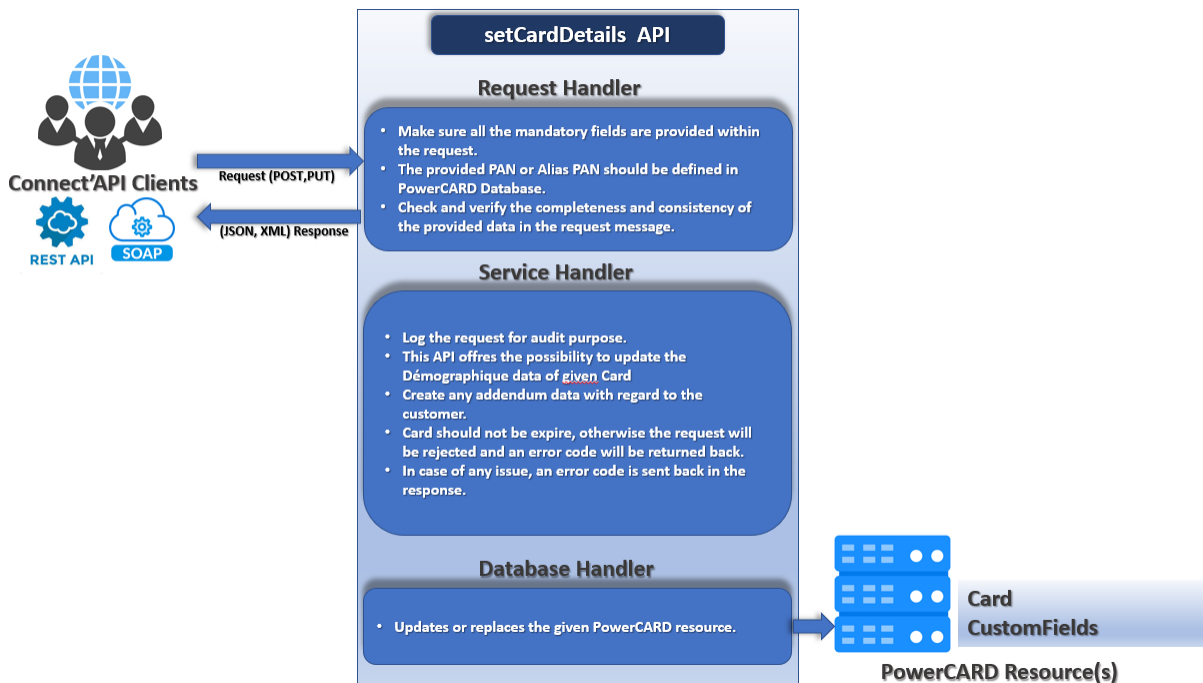
Figure 3: setCardDetails process
