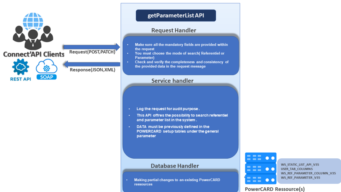
Figure 34: GetParameterList process
