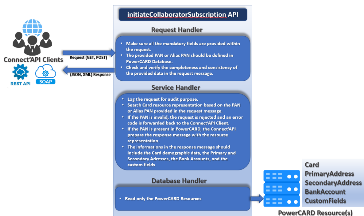
Figure 74: initiateCollaboratorSubscription process
