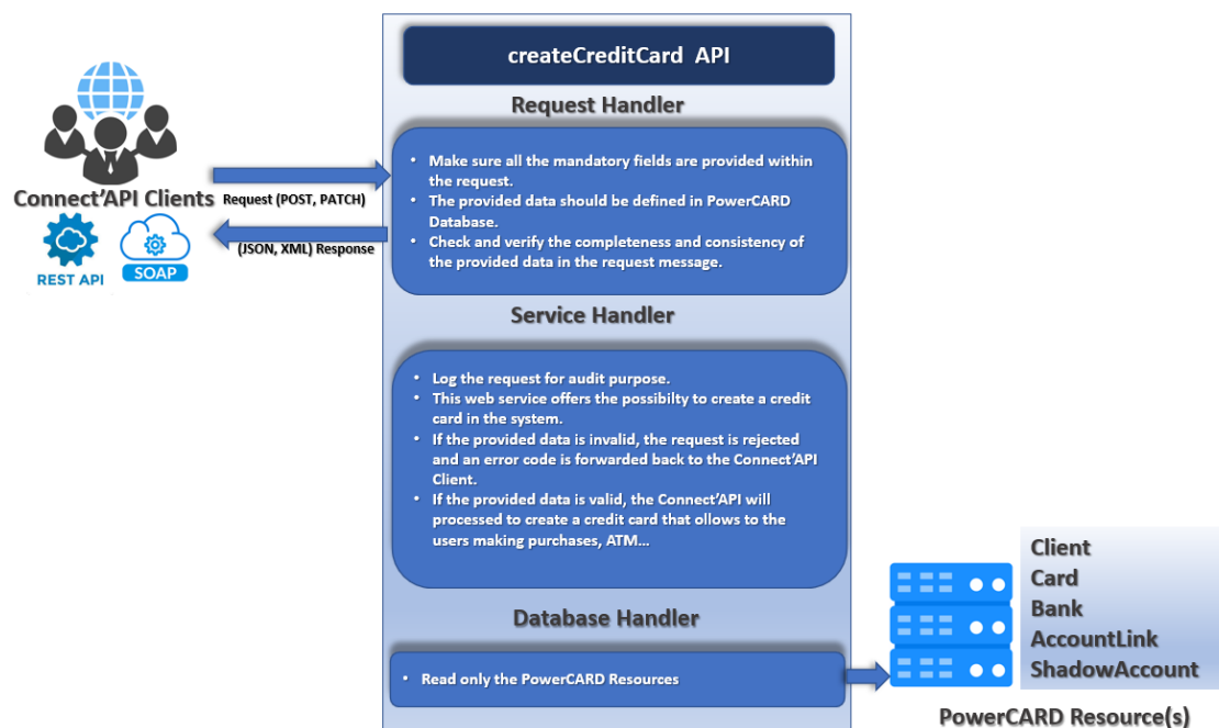
Figure 58: createCreditCard process
