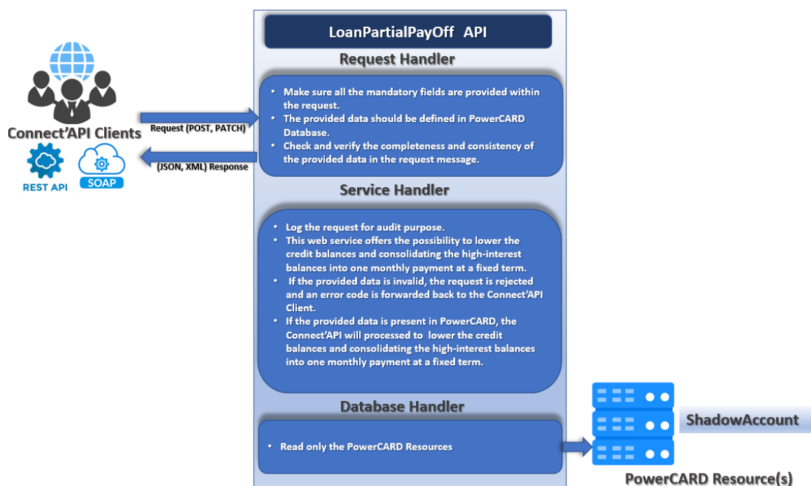
Figure 76: LoanPartialPayOff
