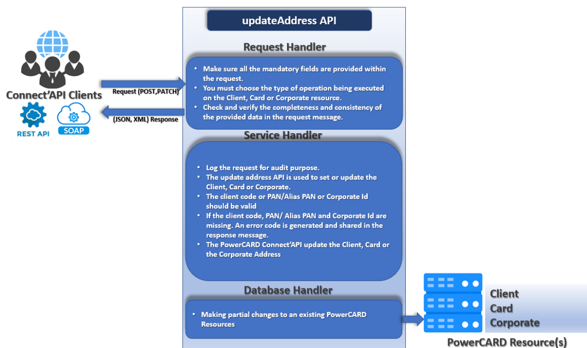
Figure 31: updateAddress process
