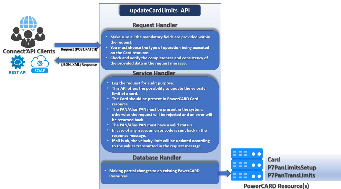
Figure 24: updateCardLimits process
