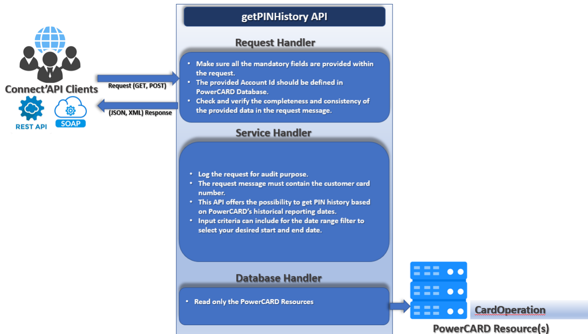
Figure 30: getPINHistory process
