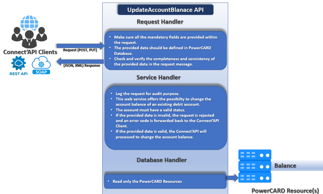
Figure 65: updateAccountBalance process
