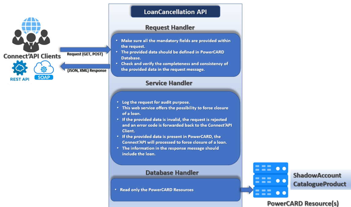
Figure 79: LoanCancellation process
