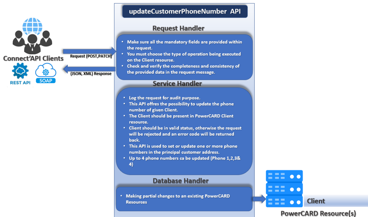
Figure 14: updateCustomerPhoneNumber process
