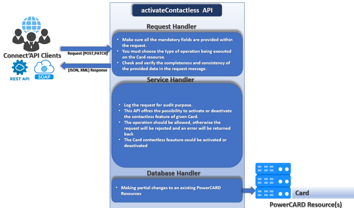
Figure 32: activateContactless process
