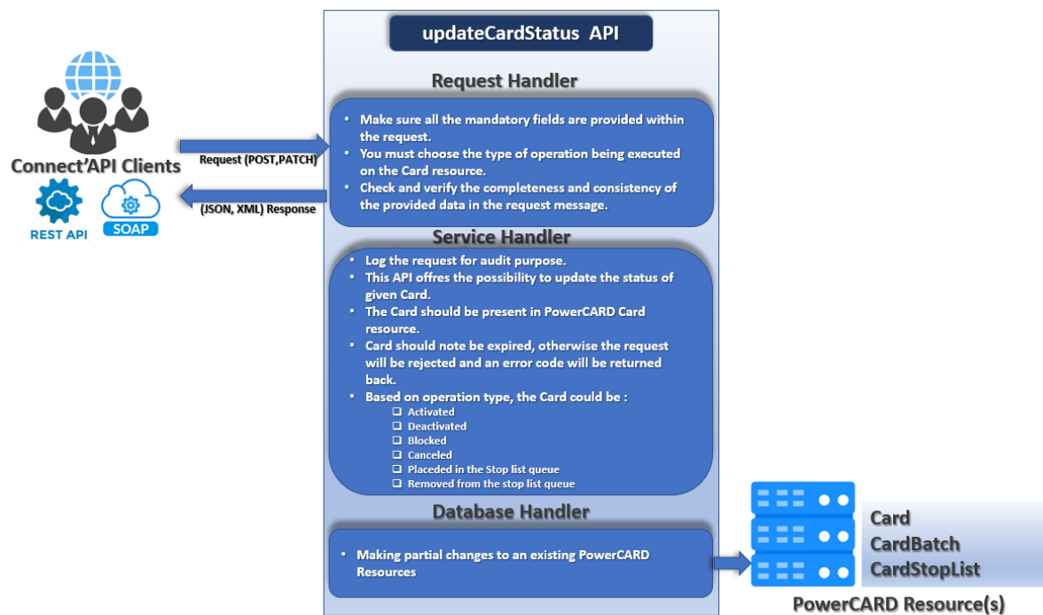
Figure 5: updateCardStatus process
