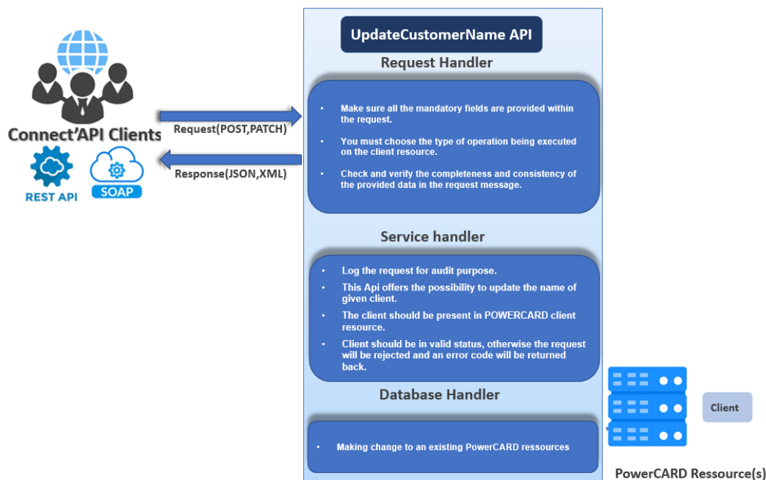
Figure 38: updateCustomerName process
