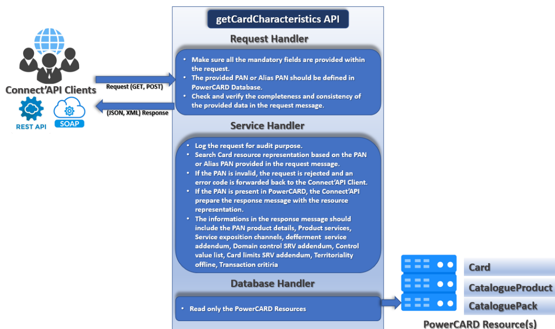
Figure 43: getCardCharacteristics
