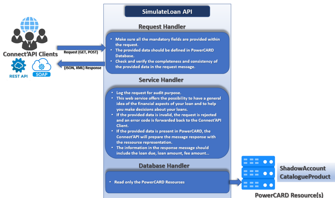
Figure 80: SimulateLoan process
