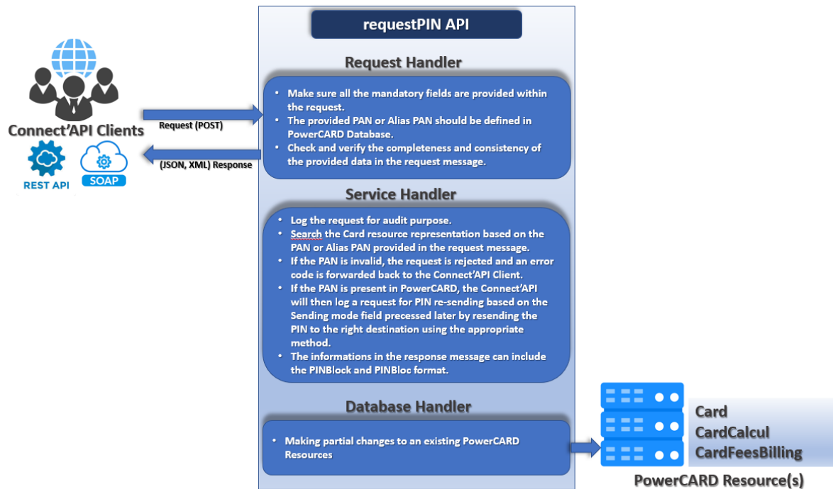
Figure 9: requestPIN process
