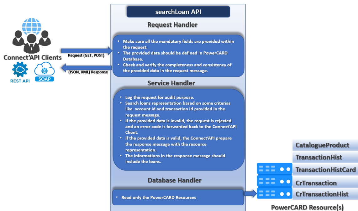
Figure 46: searchLoan process
