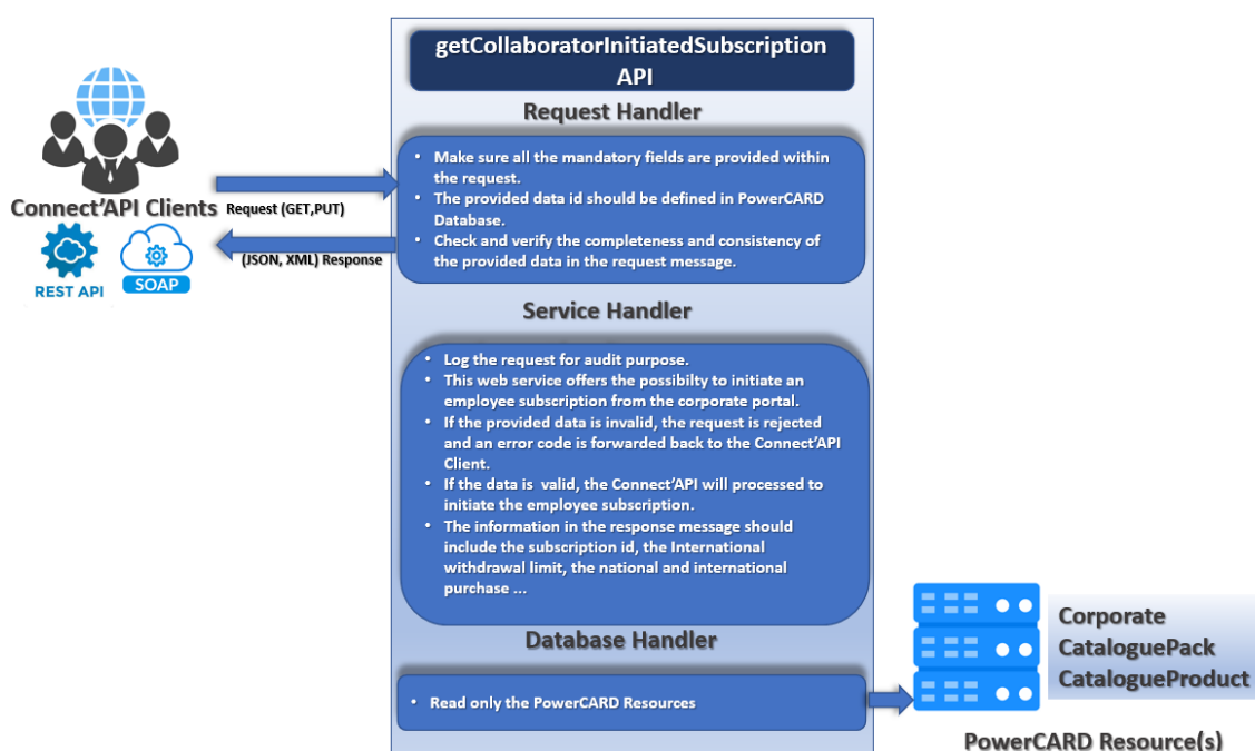
Figure 68: getCollaborationInitiatedSubscription process
