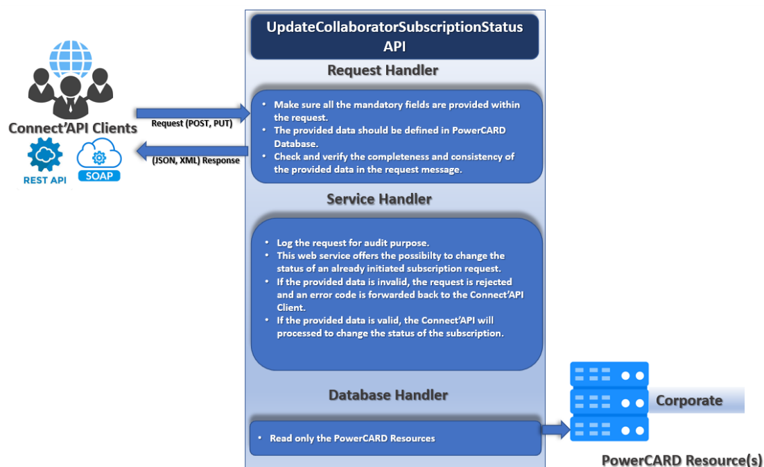
Figure 73: updateCollaboratorSubscriptionStatus process
