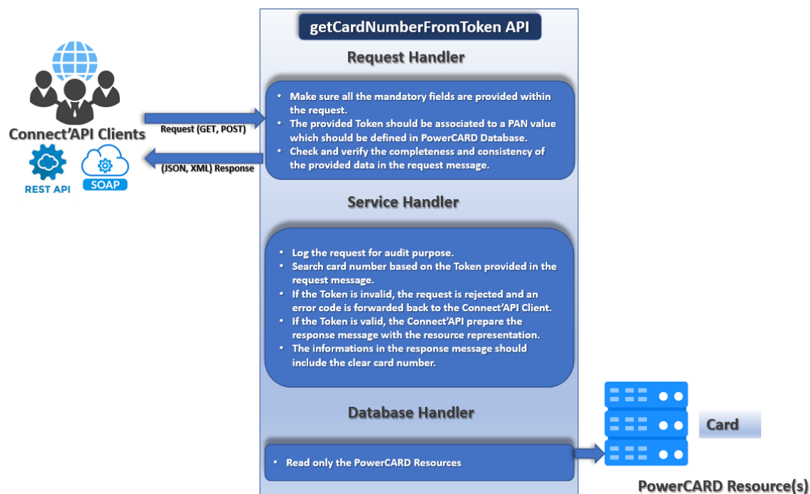
Figure 44: getCardNumberFromToken process
