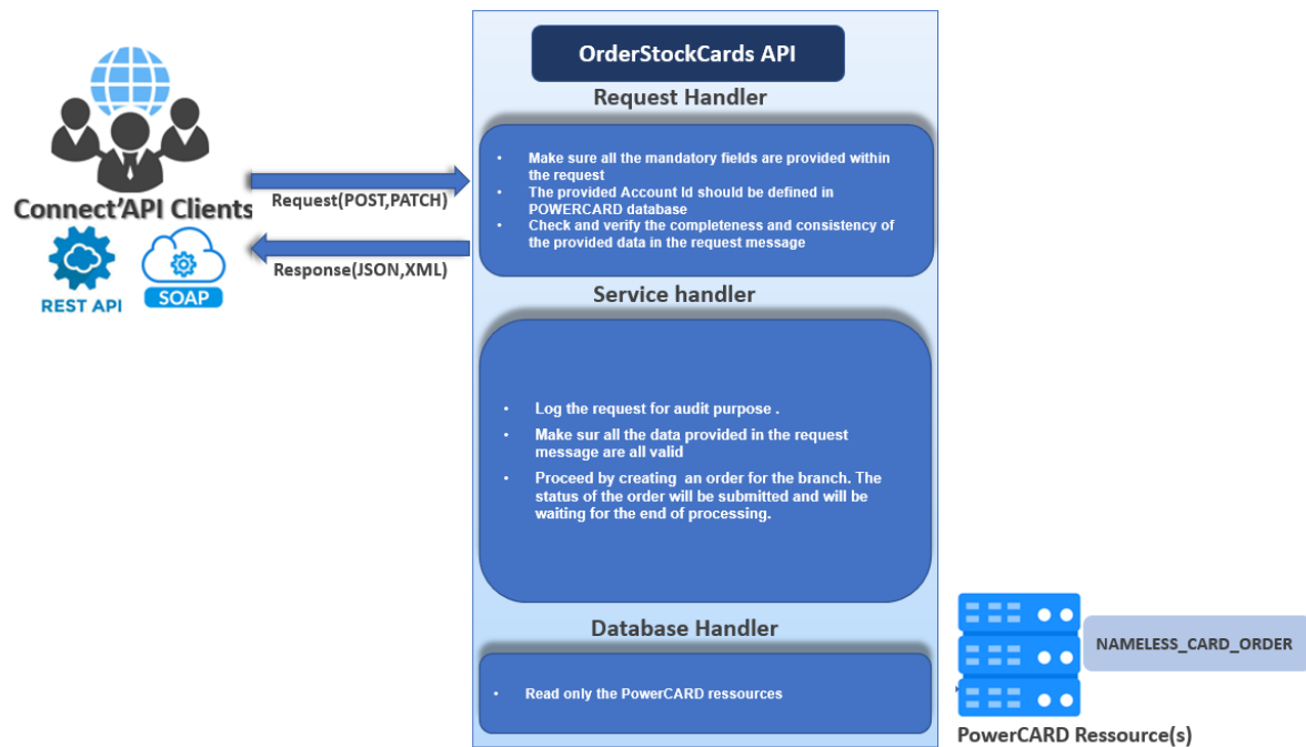
Figure 35: orderStockCards process
