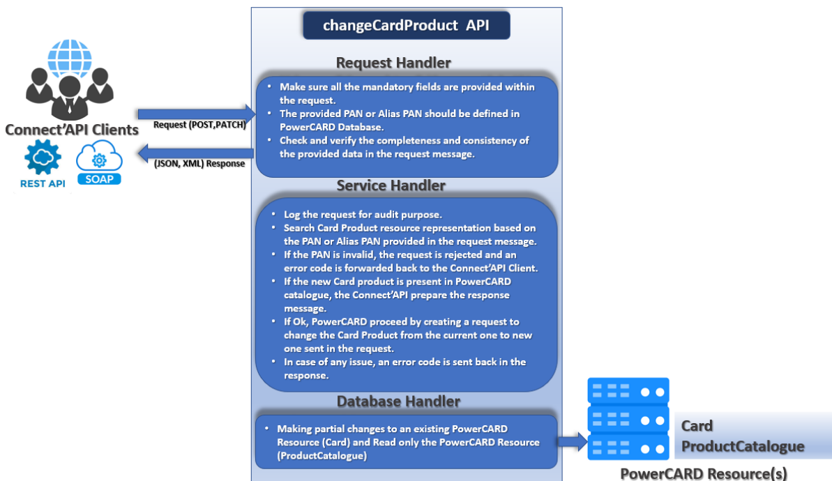
Figure 8: changeCardProduct process
