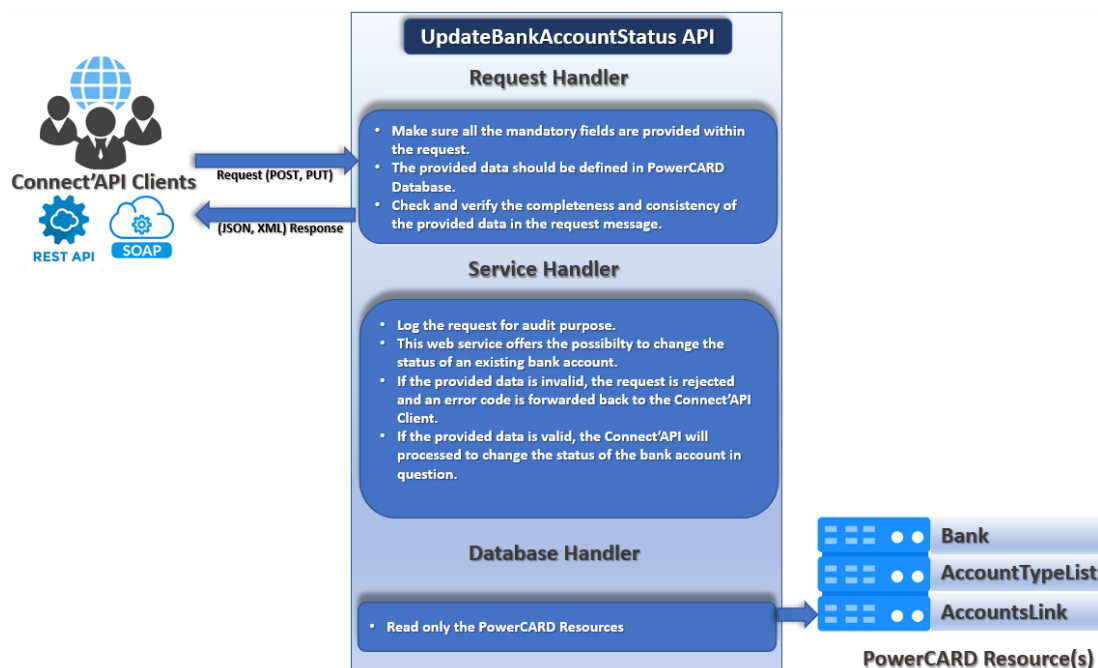
Figure 50: updateBankAccountStatus process
