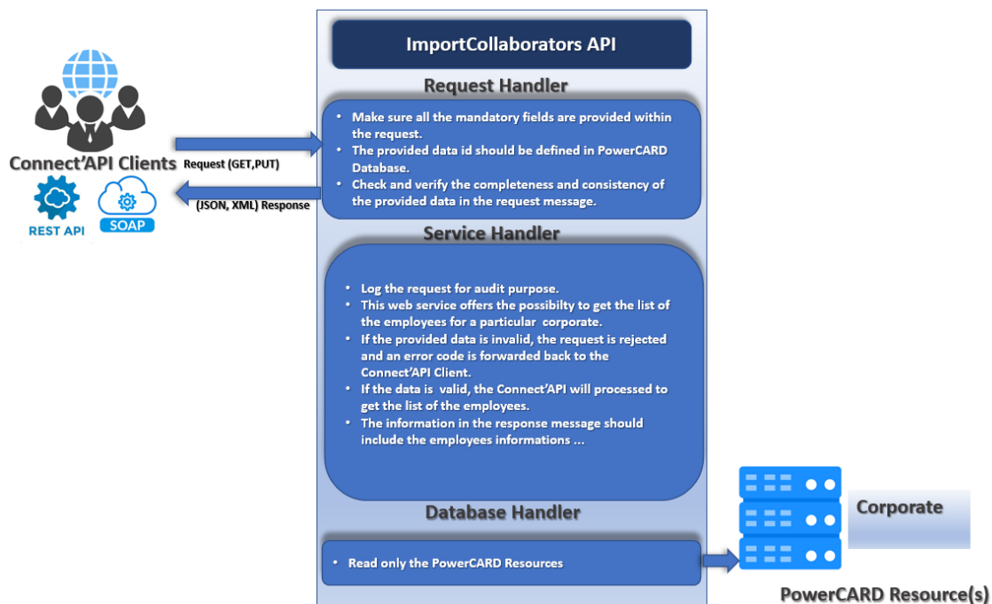
Figure 71: ImportCollaborators process
