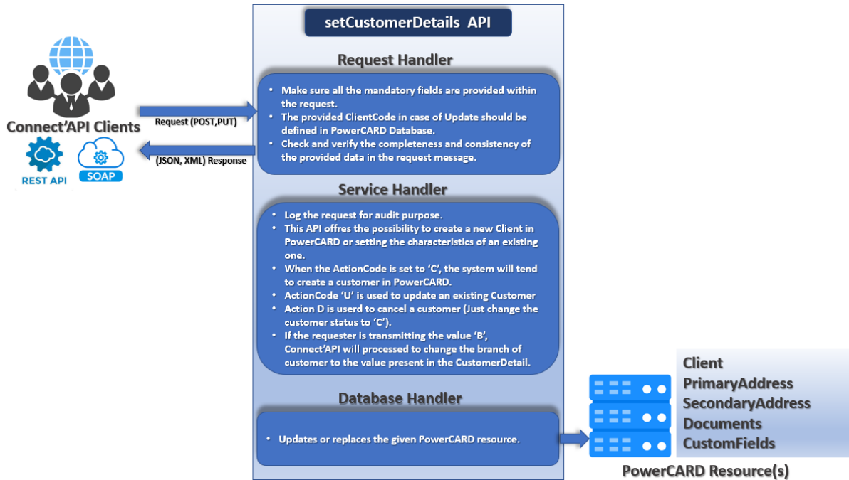
Figure 12: setCustomerDetail process
