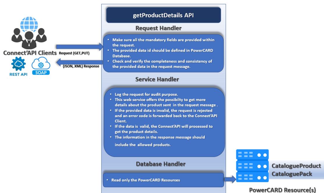
Figure 62: getProductDetails process
