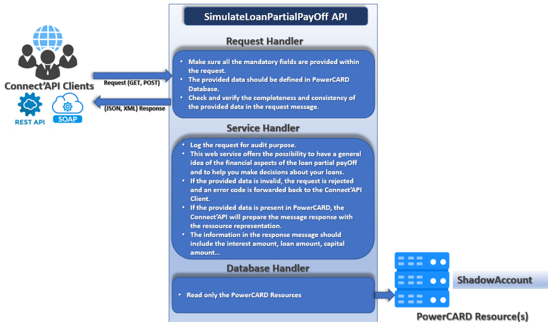
Figure 82: SimulateLoanPartialPayOff process
