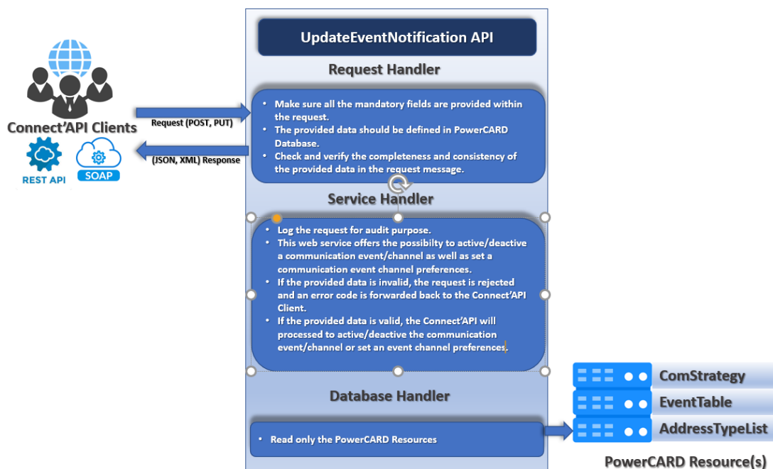
Figure 72: updateEventNotification process
