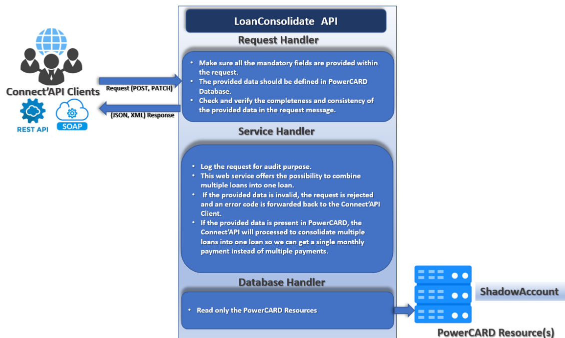
Figure 78: LoanConsolidate process
