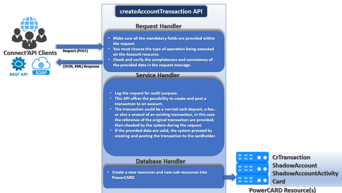
Figure 18: createAccountTransaction process
