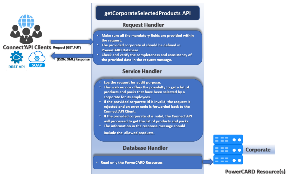
Figure 61: getCorporateSelectedProducts process
