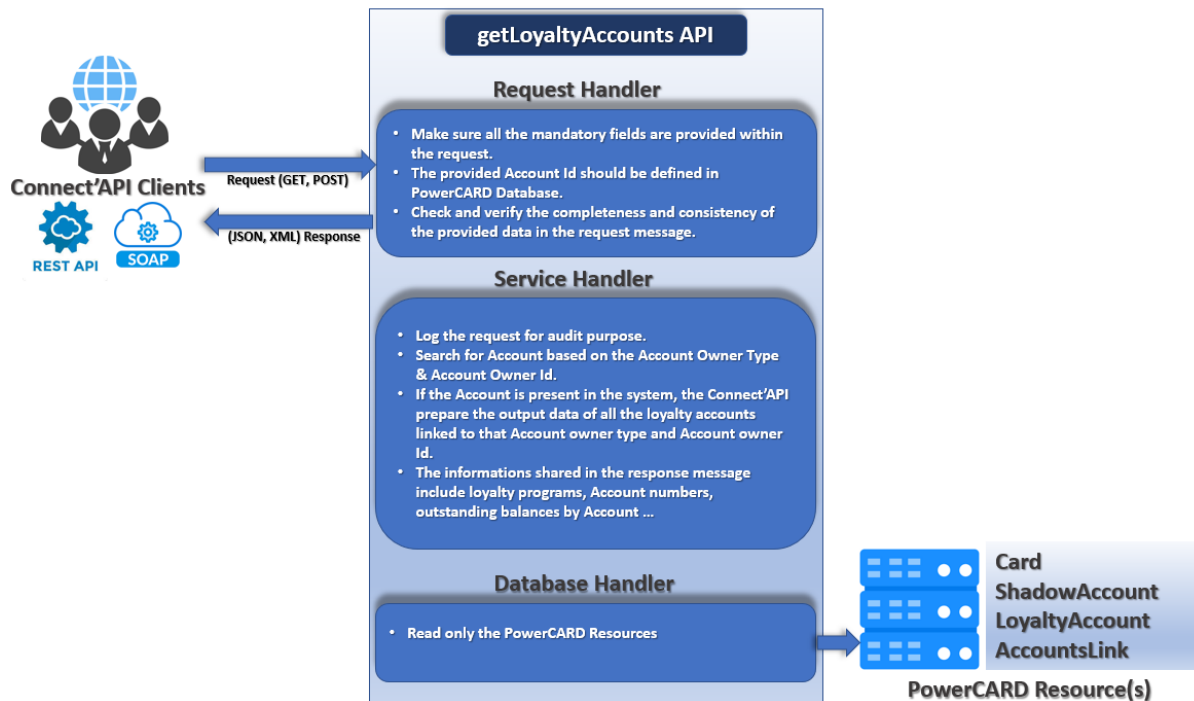
Figure 20: getLoyaltyAccounts process
