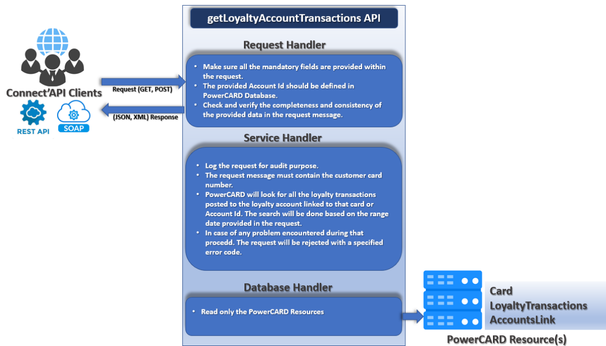
Figure 22: getLoyaltyAccountTransaction process
