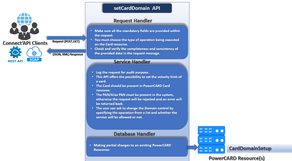
Figure 27: setCardDomain process
