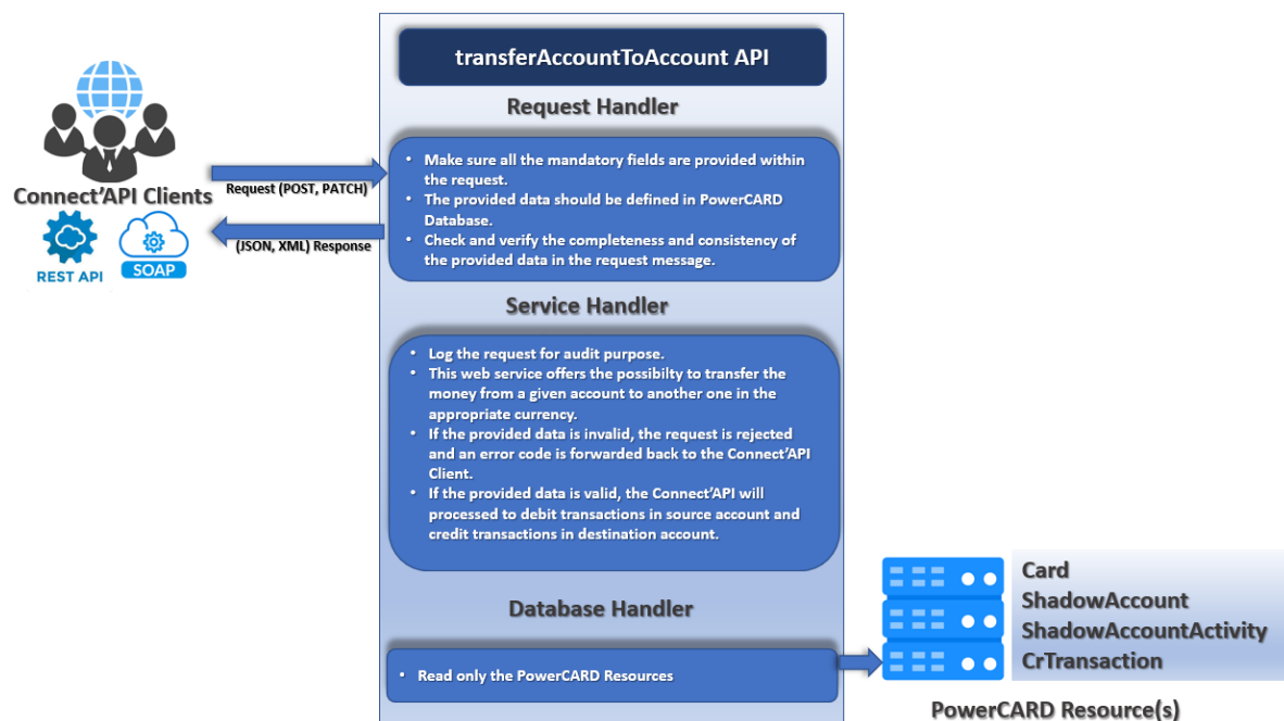
Figure 53: transferAccountToAccount process
