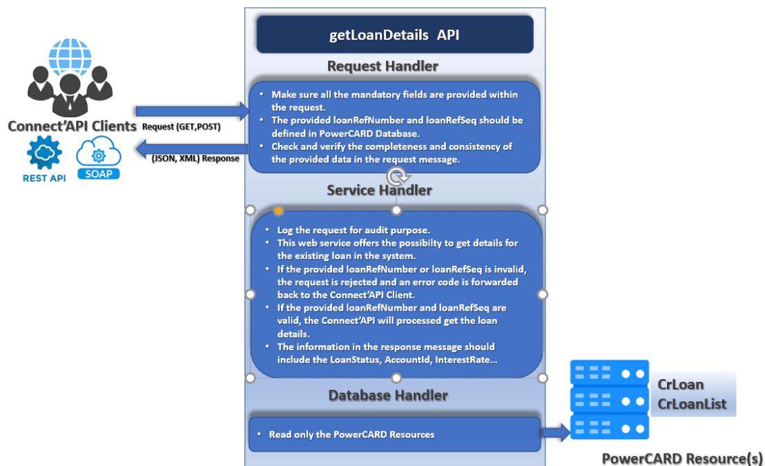
Figure 51: getLoanDetails process
