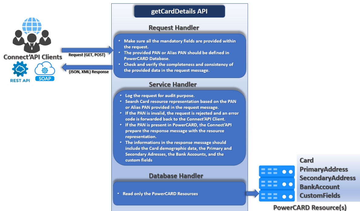
Figure 1: getCardDetails process
