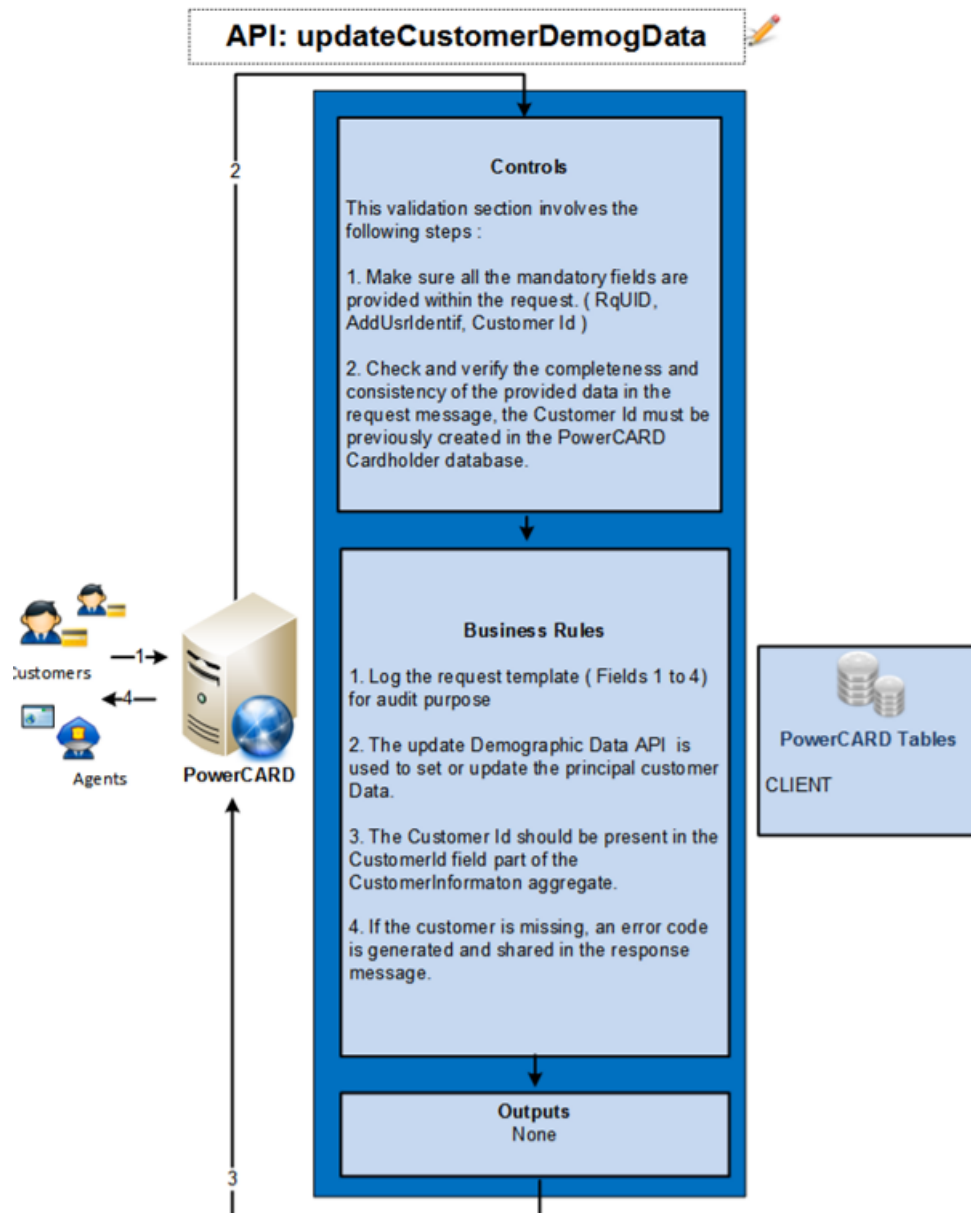
Figure 41: updateCustomerDemogData process
