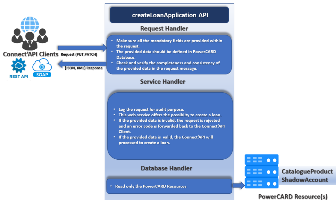
Figure 59: createLoanApplication process
