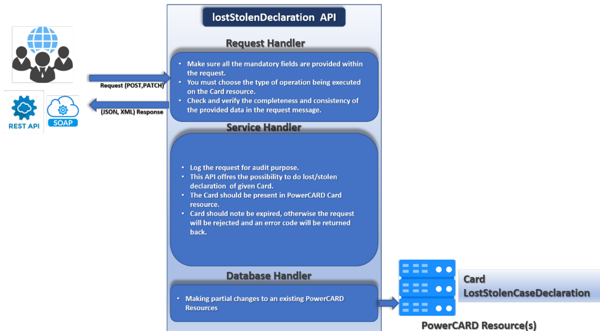
Figure 40: lostStolenDeclaration process
