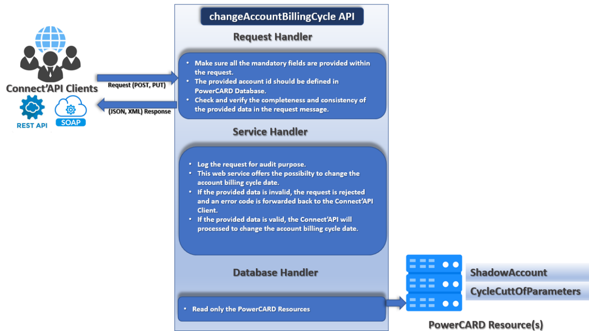
Figure 47: changeAccountBillingCycle process
