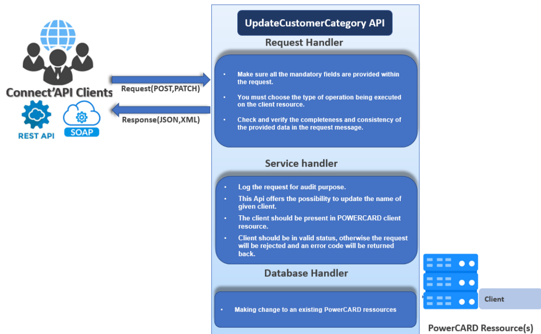
Figure 39: updateCustomerCategory
