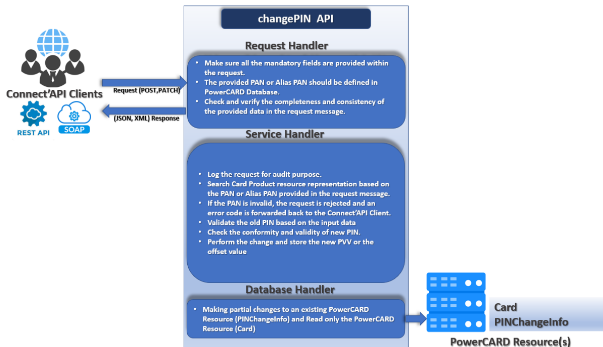
Figure 28: changePIN process
