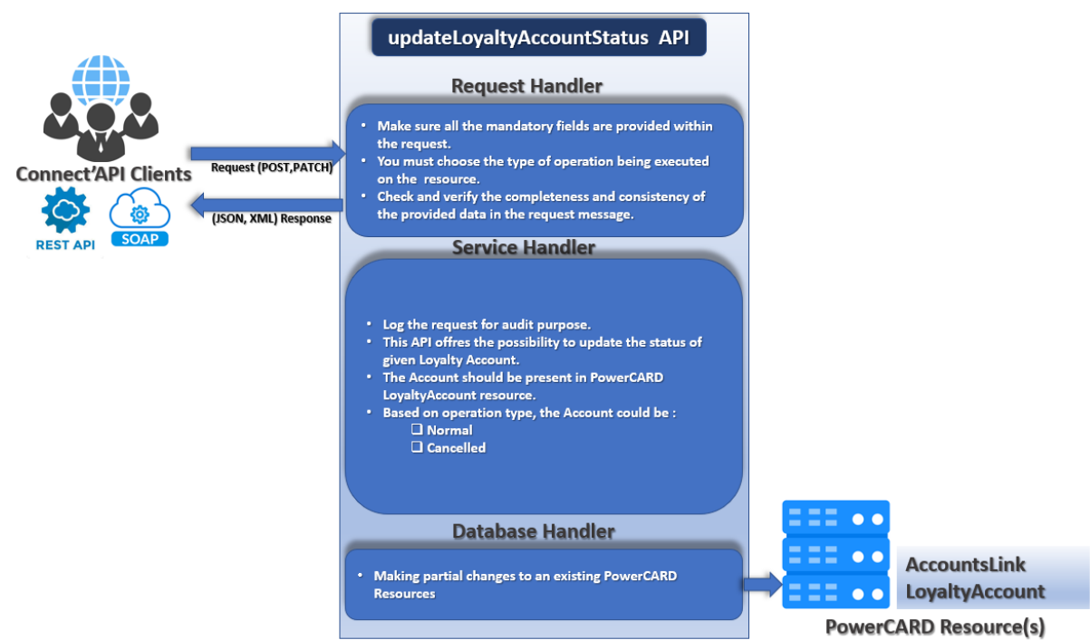
Figure 23: updateLoyaltyAccountStatus process
