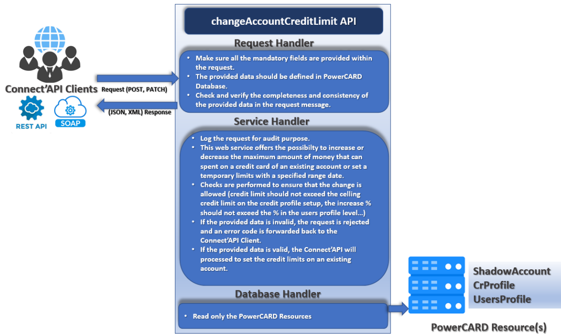
Figure 56: changeAccountCreditLimit process
