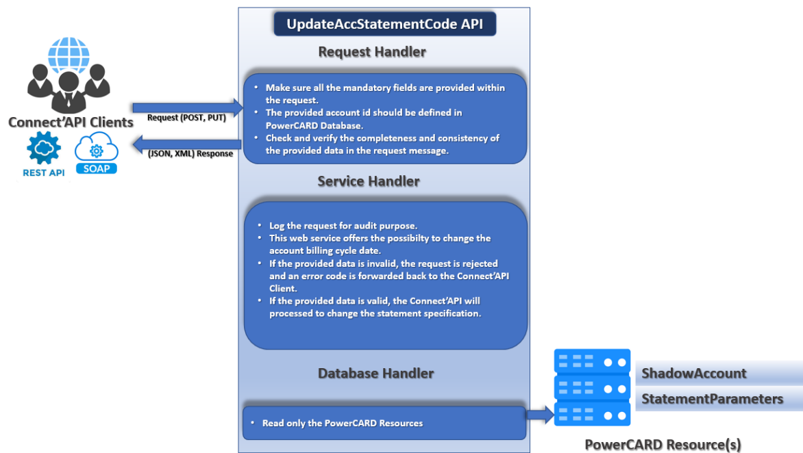
Figure 49: updateAccStatementCode process
