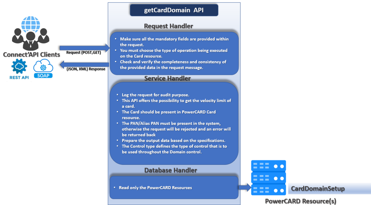
Figure 26: getCardDomain process
