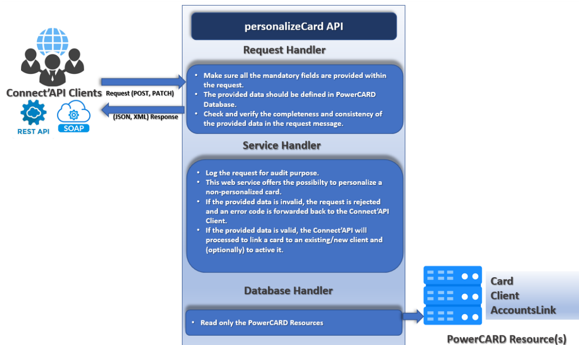
Figure 52: personalizeCard process
