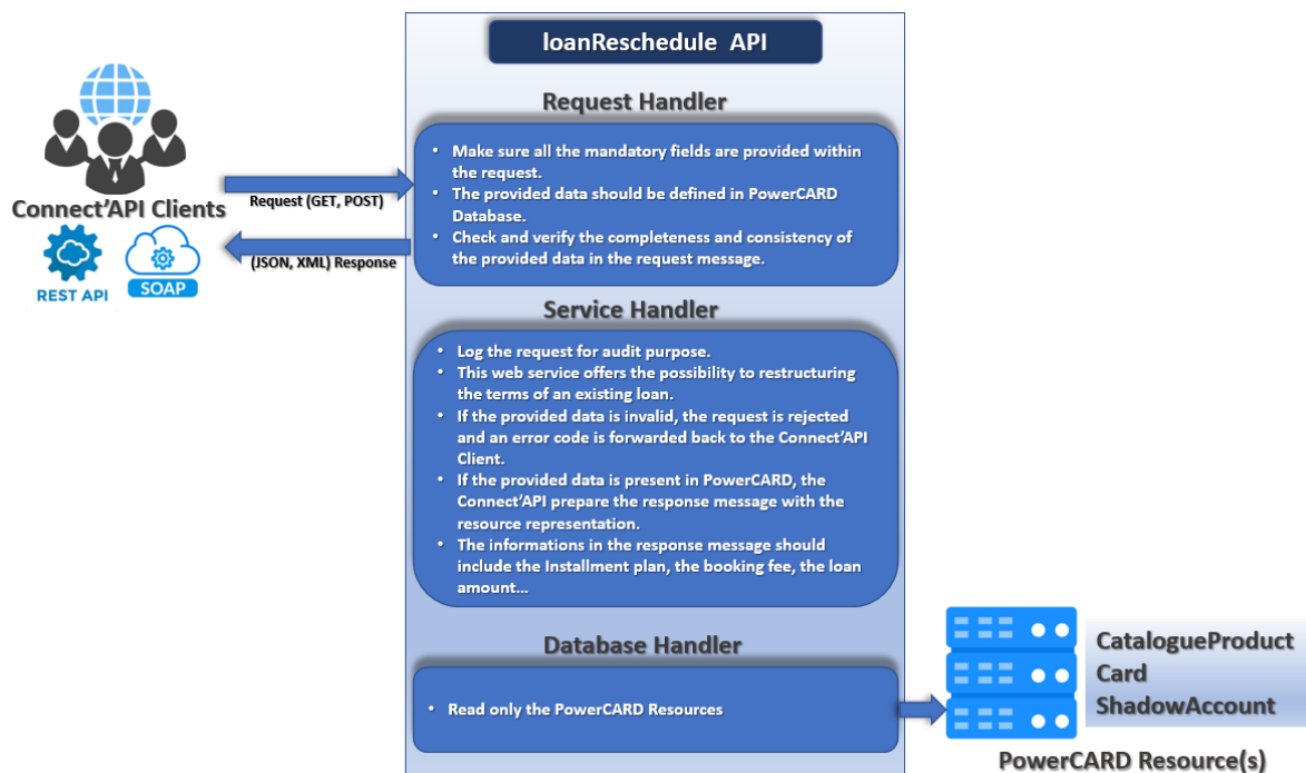
Figure 75: loanReschedule process
