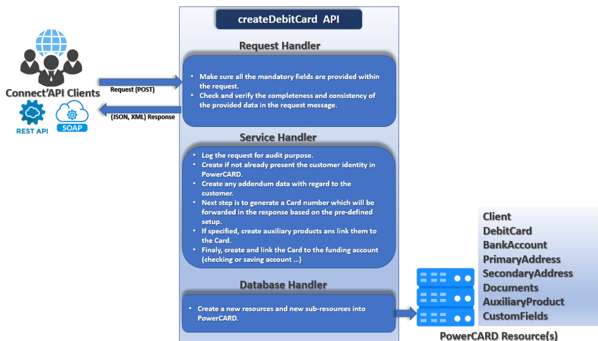
Figure 2: createDebitCard process
