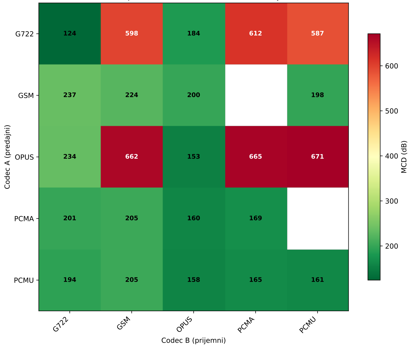
Mel Cepstral Distortion matrica (niže = bolje)
