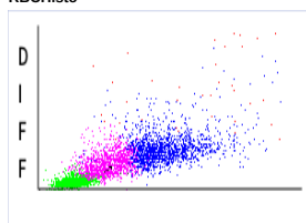
S90_S90DDIFFSca
