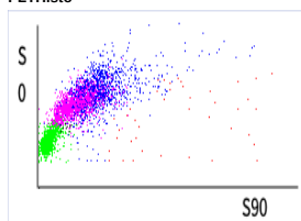
S0_S90Scattergr
