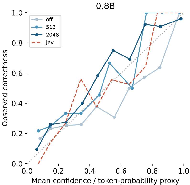
Exploratory reliability · valid answers with an available score Qwen: emitted answer-token probability; Jev: returned confidence (different definitions)
