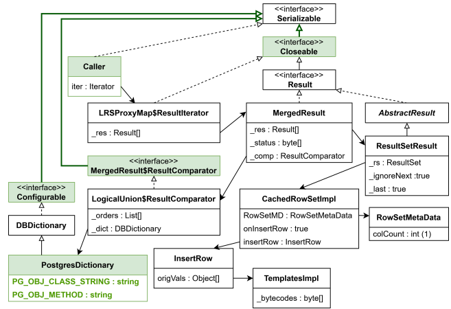
Figure 6: Payload visualization for dormant OpenJPA gadget chain. Modifications are highlighted in green. Making LRSPProxyMap$ResultIterator , MergedResult , and ResultSetResult serializable requires only the addition of Serializable to OpenJPA 's Closeable since all three gadgets inherit from it. It illustrates quite well how changing the serializability of a single interface (or class) can have a substantial impact on its descendants. Additionally, we provide transitive serializability via Configurable and MergedResults$ResultComparator to PostgresDictionary and LogicalUnion$ResultComparator , respectively.
