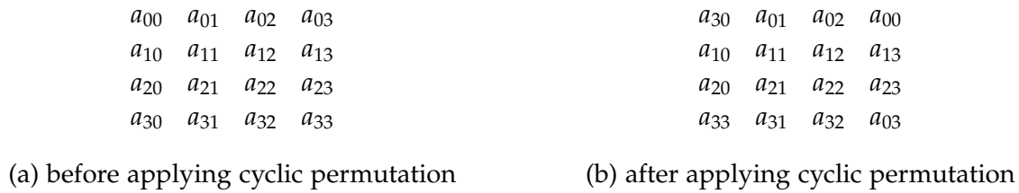
Figure 2: Applying the cyclic permutation a_{00} \rightarrow a_{03} \rightarrow a_{33} \rightarrow a_{30} \rightarrow a_{00} to a 4 \times 4 matrix.
