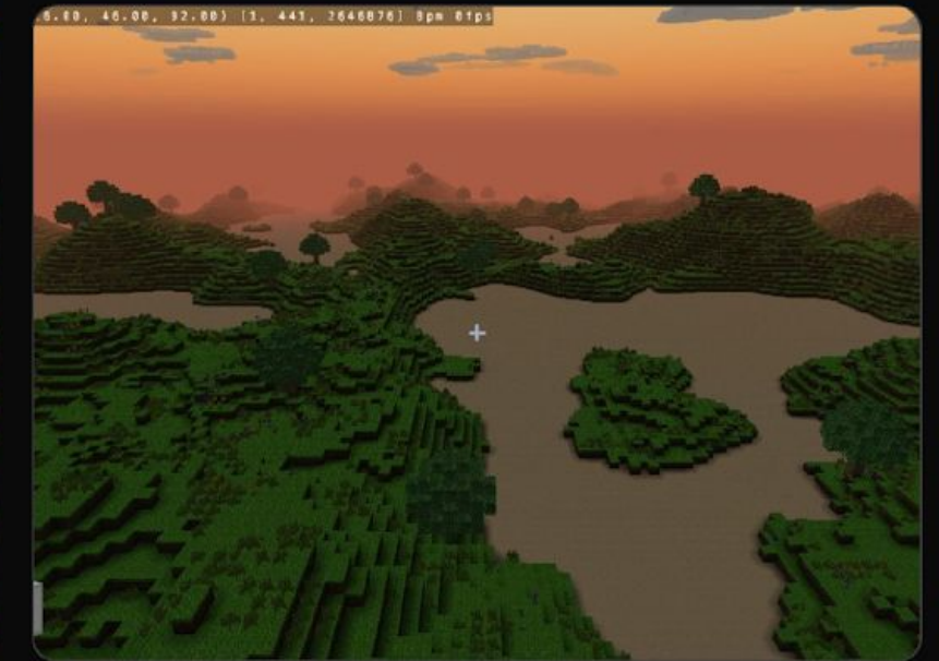
RUST PORT
