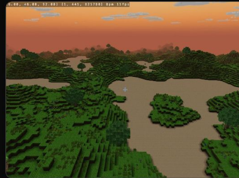
C ORIGINAL
