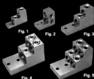
ALUMINIUM MECHANICAL LUGS (PB TYPE)
