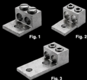
ALUMINIUM MECHANICAL LUGS (AU TYPE)
