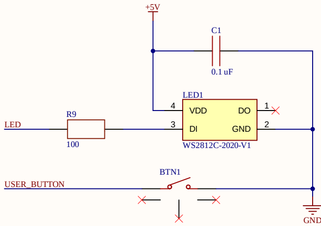
USER LED & BUTTON
