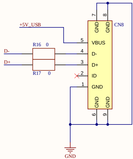
USB CONNECTOR
