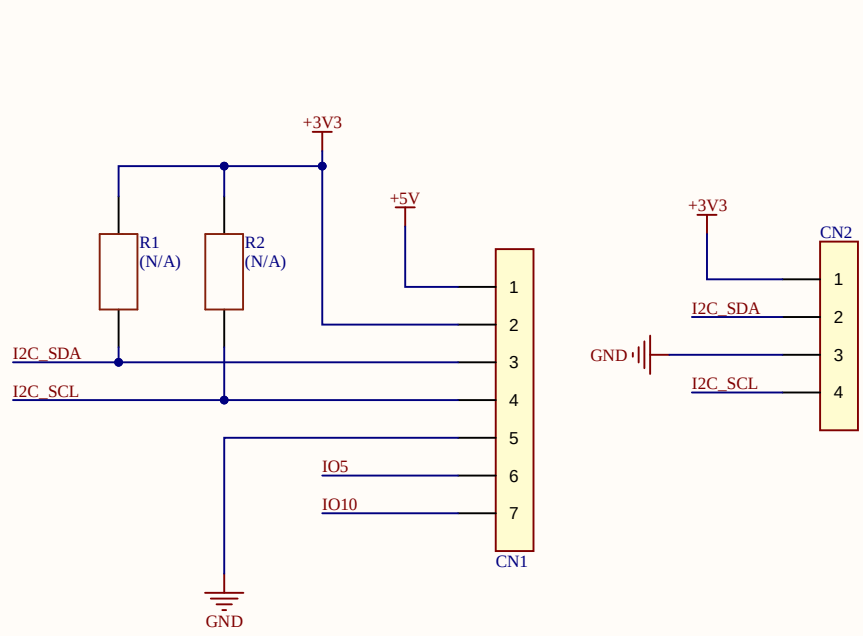
ONBOARD CONNECTORS
