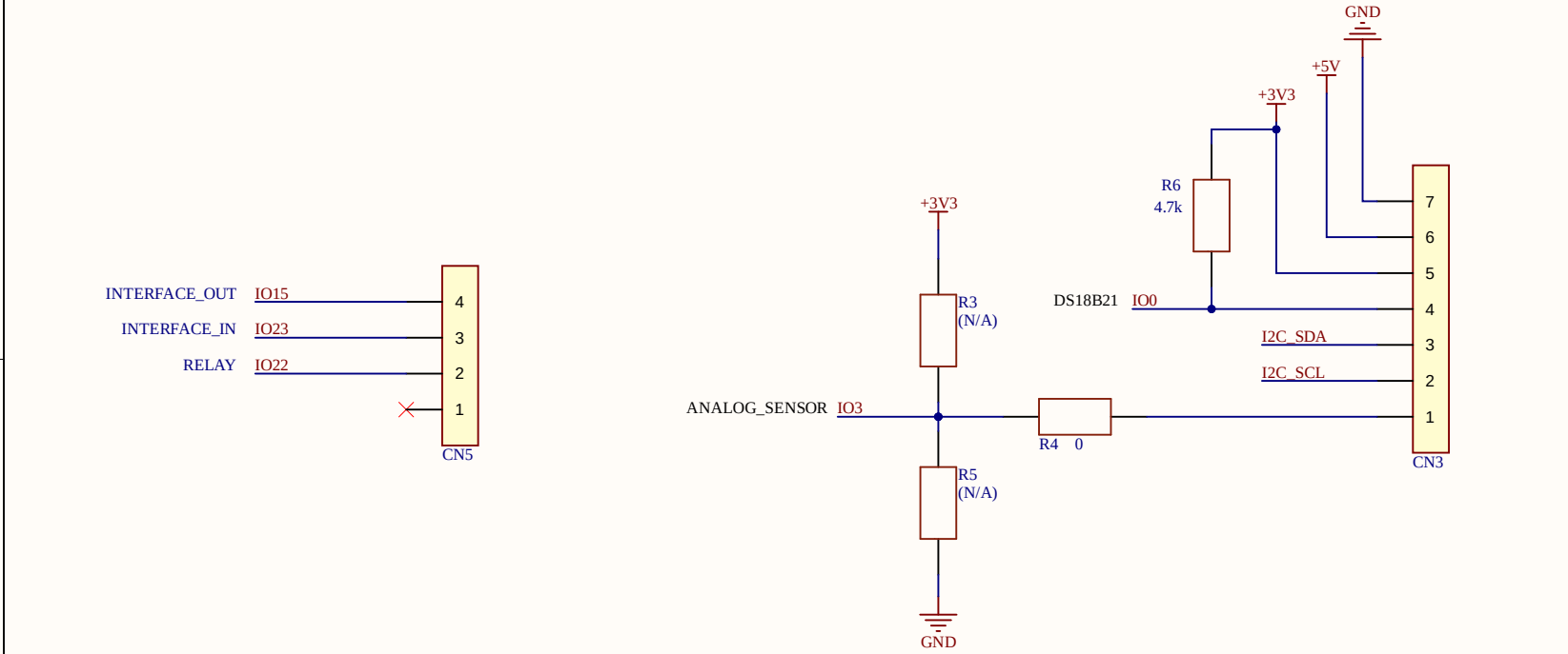
INTERBOARD CONNECTORS
