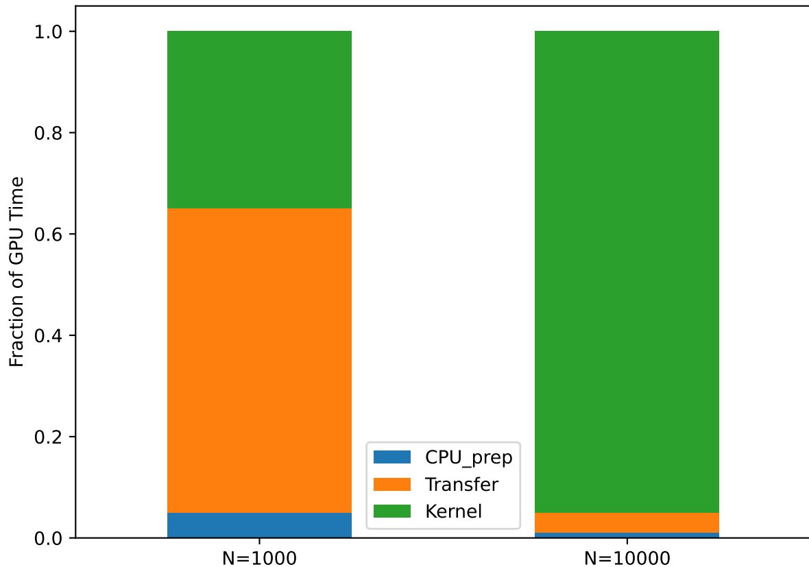
SpMV GPU Overhead Breakdown
