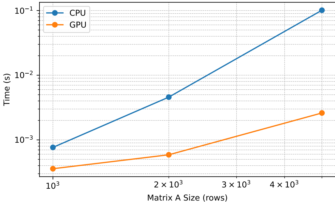
SpGEMM: CPU vs GPU Time
