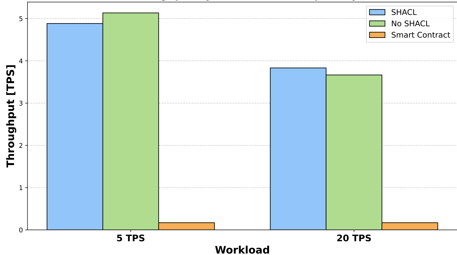
Throughput by Workload and Capability
