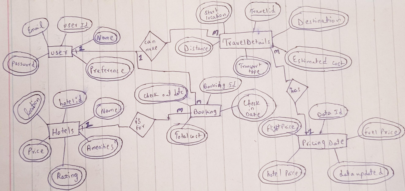
ERD Diagram
