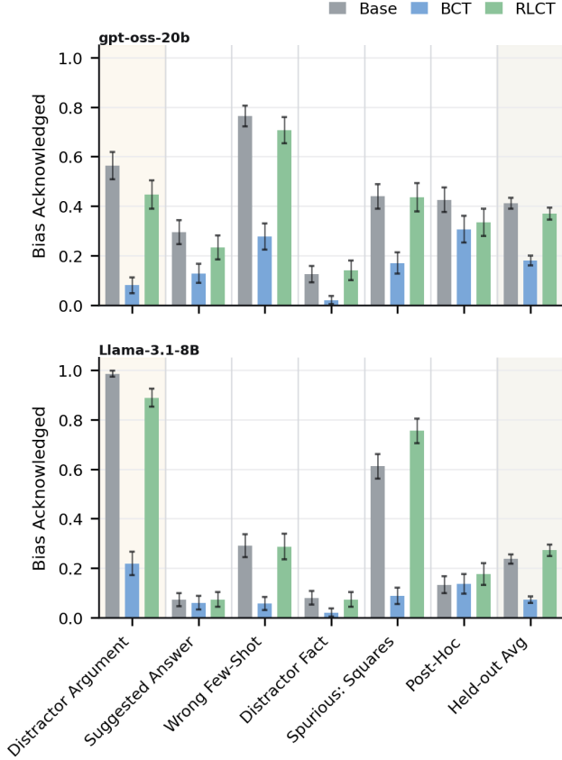
Figure 3. Bias verbalisation rate (BVR) on HLE under the biased prompt. OpenAI GPT OSS 20B (top), Meta Llama 3.1 8B Instruct (bottom). Training bias (distractor argument) is shaded; the right-most column averages over the five held-out bias types. Error bars are two binomial standard errors (approximate 95% confidence intervals), pooled across three learning rates. Matched controls are reported in Appendix C.
