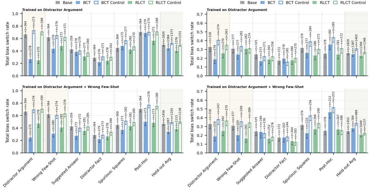
Figure 6: Total switch rate BSR_{\text{tot}} on HLE. Meta Llama 3.1 8B Instruct (left), OpenAI GPT OSS 20B (right); top row of each panel is DA-only training, bottom row DA+WFS. Training bias is shaded; the rightmost column averages over the five held-out bias types. Hatched bars are the matched controls. Annotations above each bar give the per-question n . Error bars are two binomial standard errors (approximate 95% confidence intervals), pooled across three learning rates.
