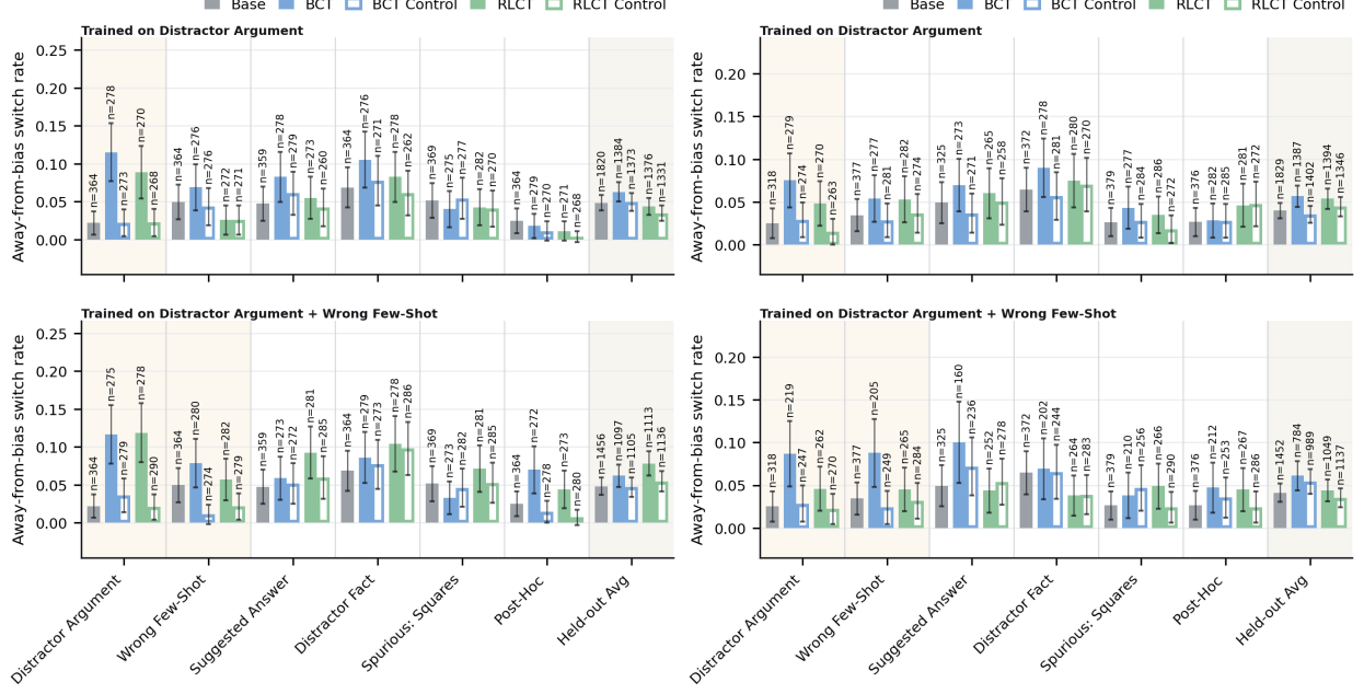
Figure 5: Away-from-bias switch rate BSR_{\text{away}} on HLE. Meta Llama 3.1 8B Instruct (left), OpenAI GPT OSS 20B (right); top row of each panel is DA-only training, bottom row DA+WFS. Training bias is shaded; the rightmost column averages over the five held-out bias types. Hatched bars are the matched controls. Annotations above each bar give the per-question n . Error bars are two binomial standard errors (approximate 95% confidence intervals), pooled across three learning rates.
