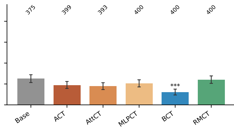
Held-out biases
