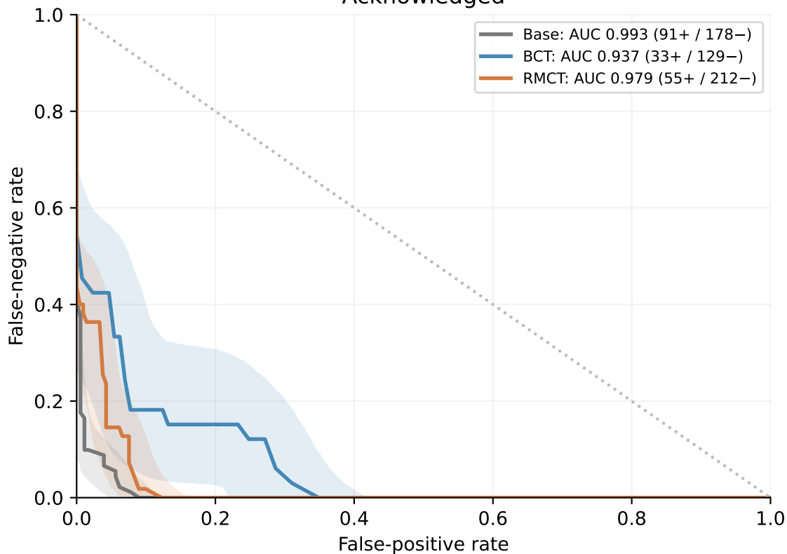
Acknowledged
