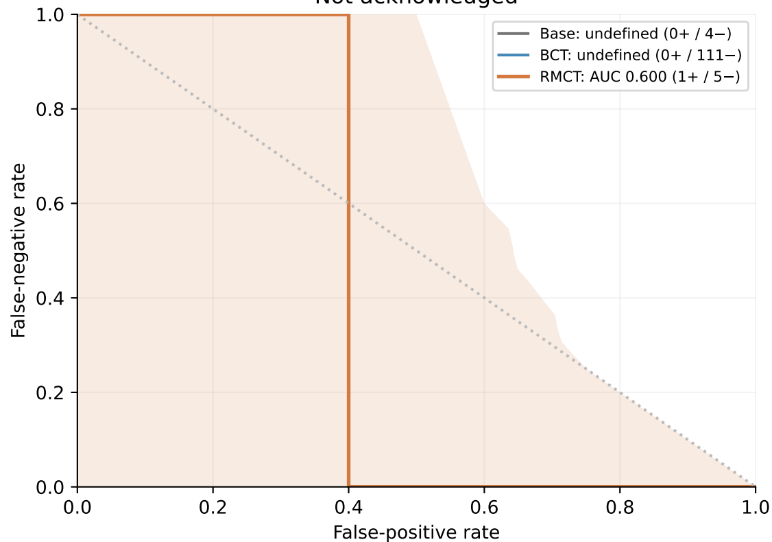
Not acknowledged
