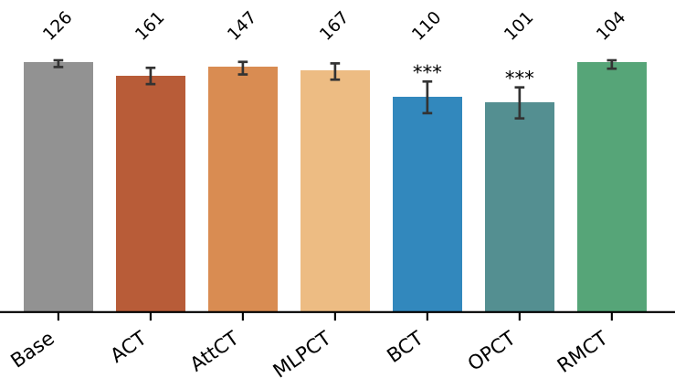
Held-out biases
