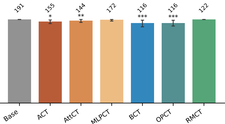
Held-out biases
