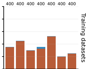
Qwen3.5-9B
