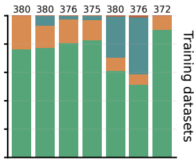
Held-out biases
