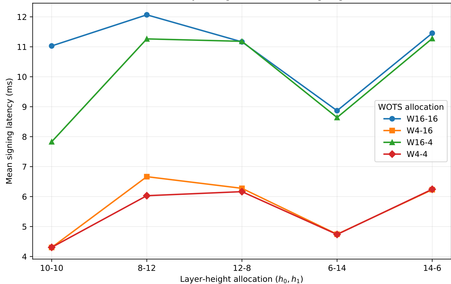
Effect of layer-height allocation on signing
