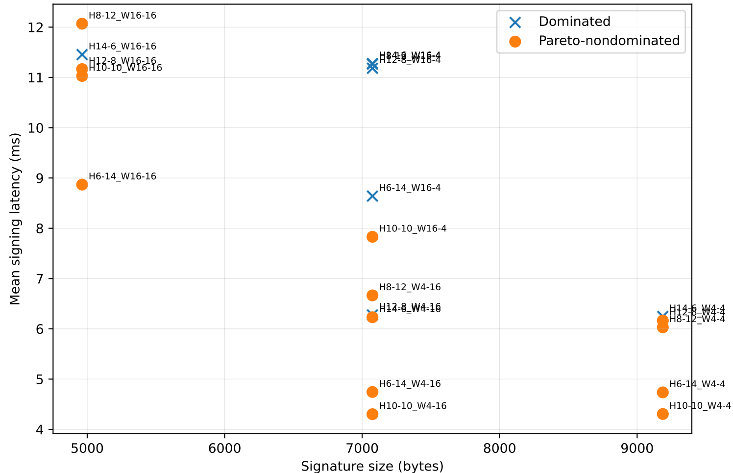
XMSSMT heterogeneous parameter trade-off
