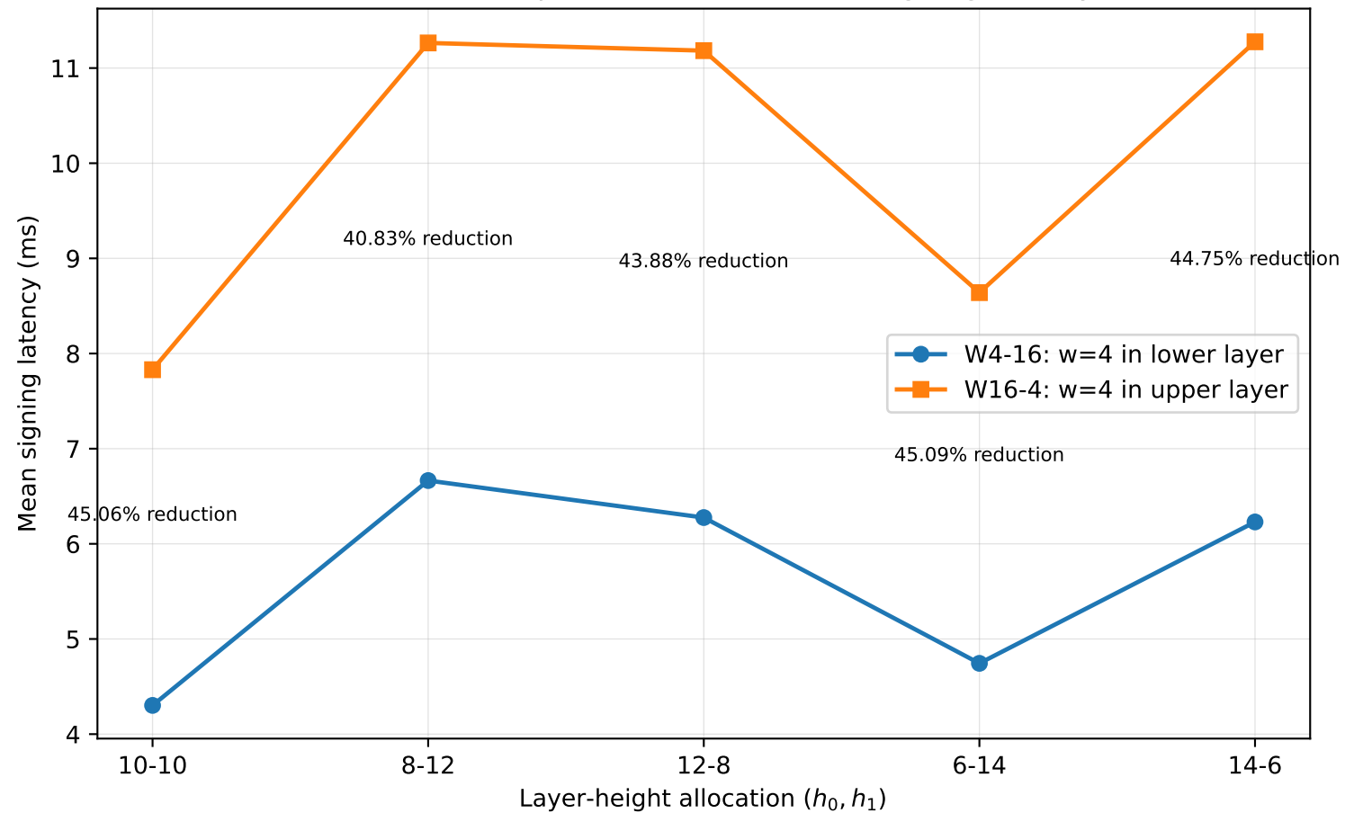
Effect of WOTS placement on XMSSMT signing latency
