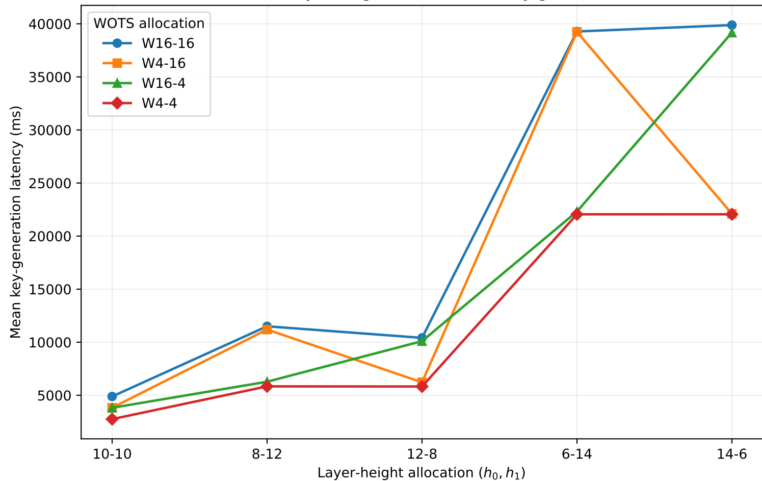
Effect of layer-height allocation on key generation
