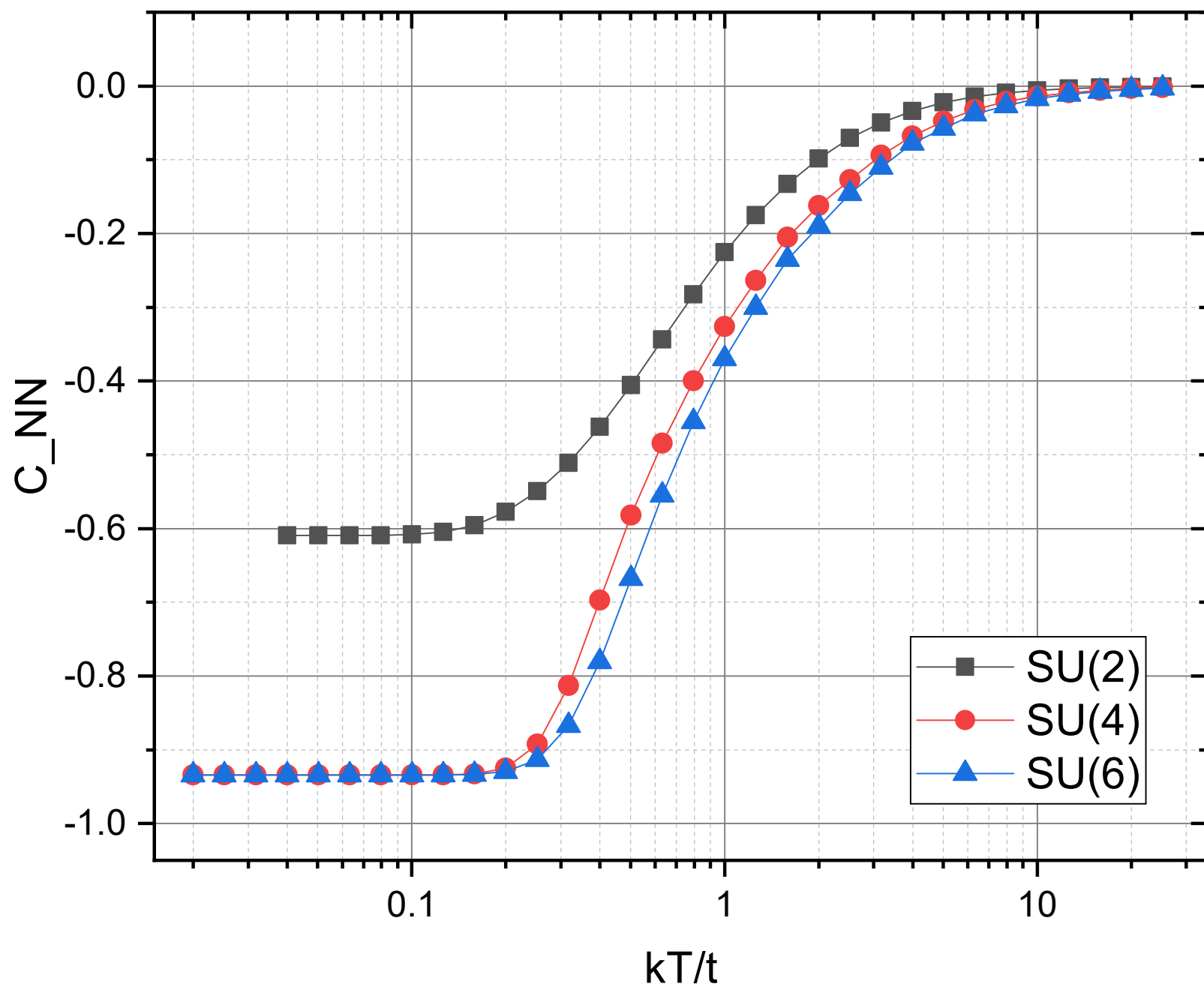
2x2 Nearest-neighbor nn-correlation @ U=15.3t \langle n \rangle = 1
