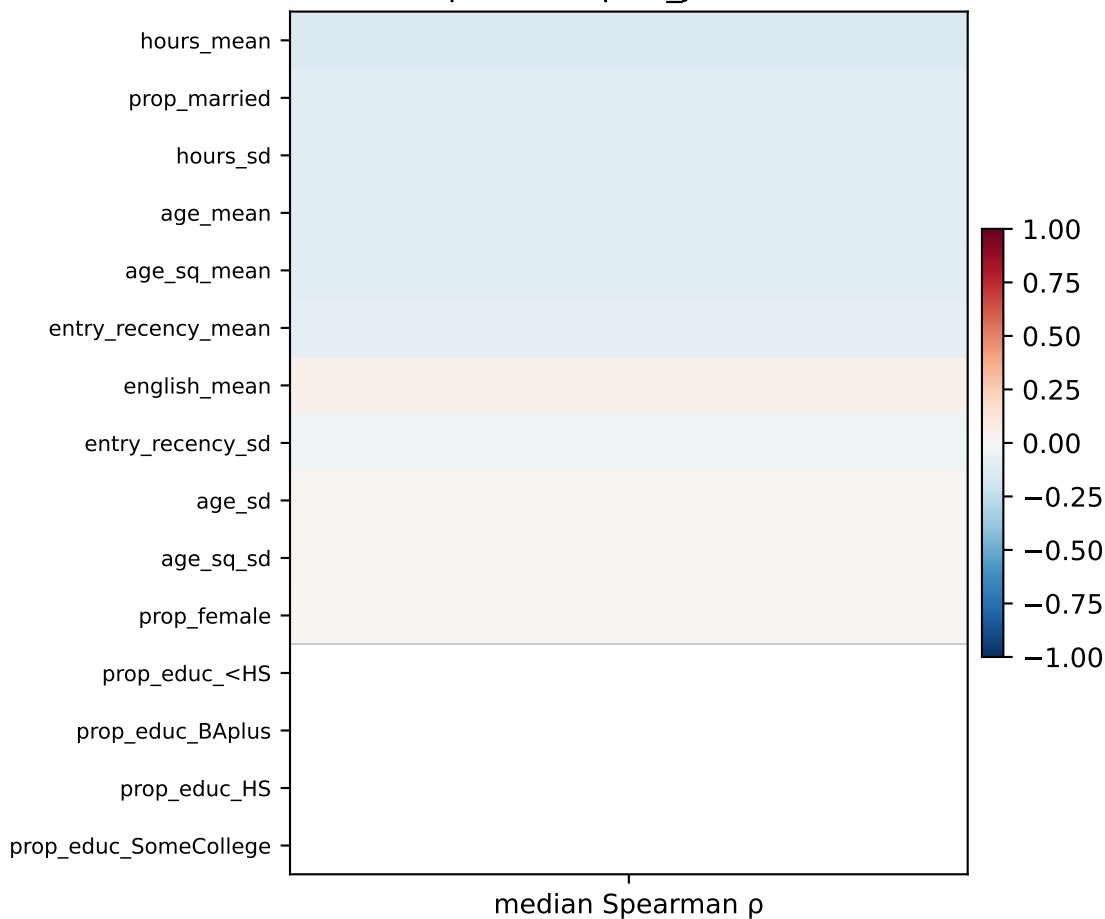
Median Spearman \rho : N_j vs X summaries
