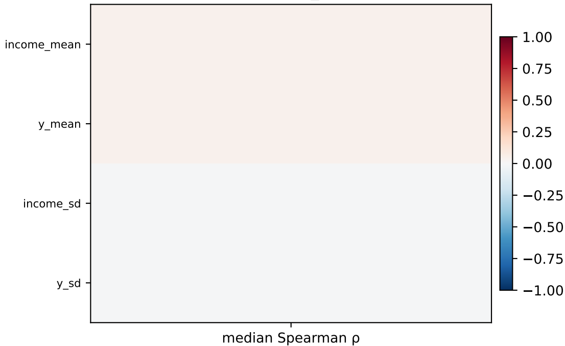
Median Spearman \rho : N_j vs Y summaries
