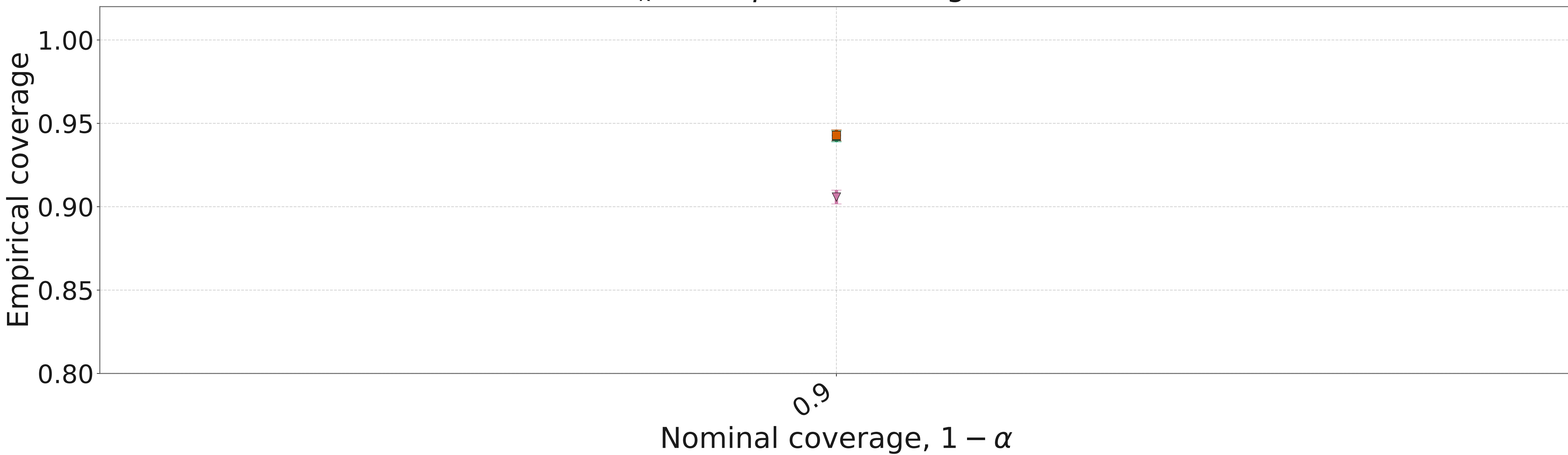
Fixed N_k = 21 , \gamma = 5 : coverage over 1 - \alpha
