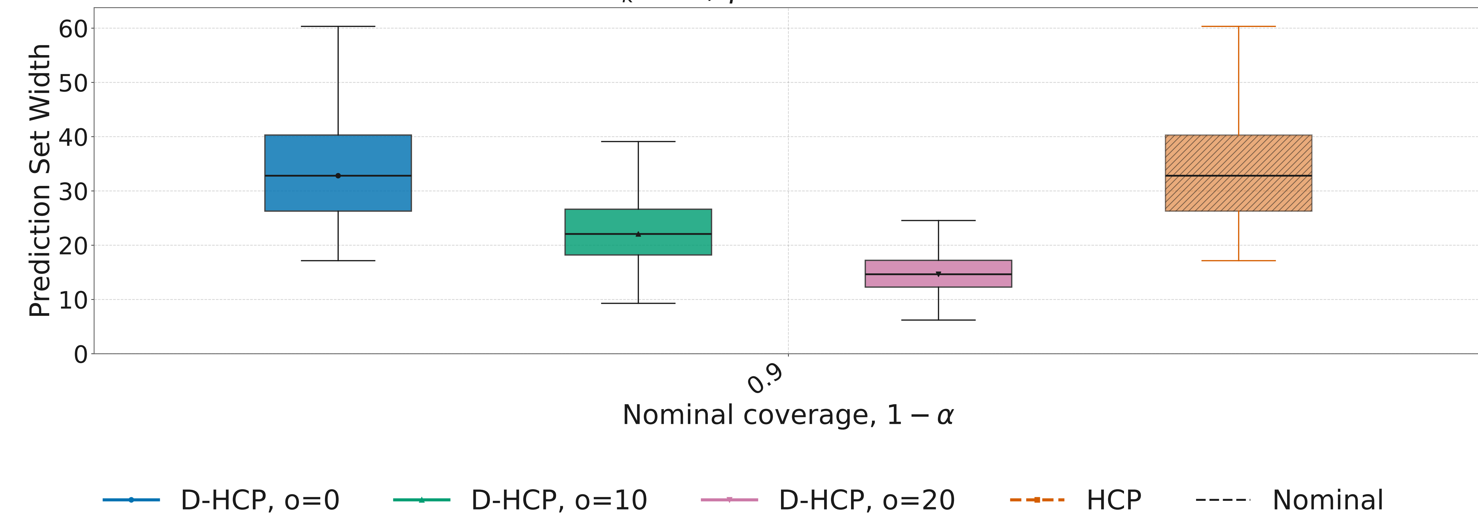
Fixed N_k = 21 , \gamma = 5 : widths over 1 - \alpha
