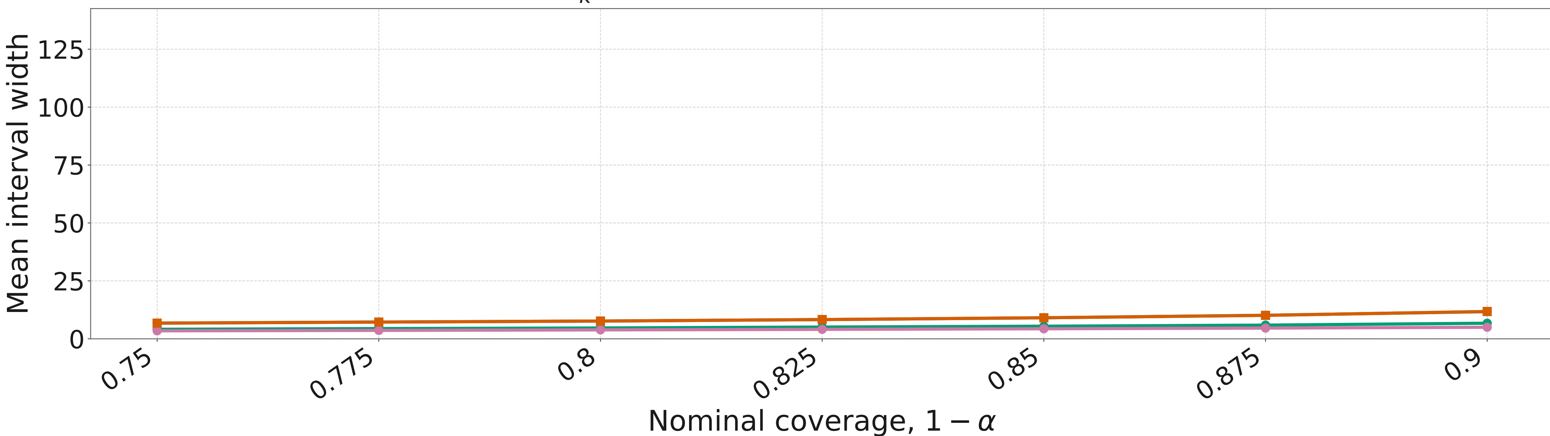
Fixed N_k = 21 : Width with standard-error bands
