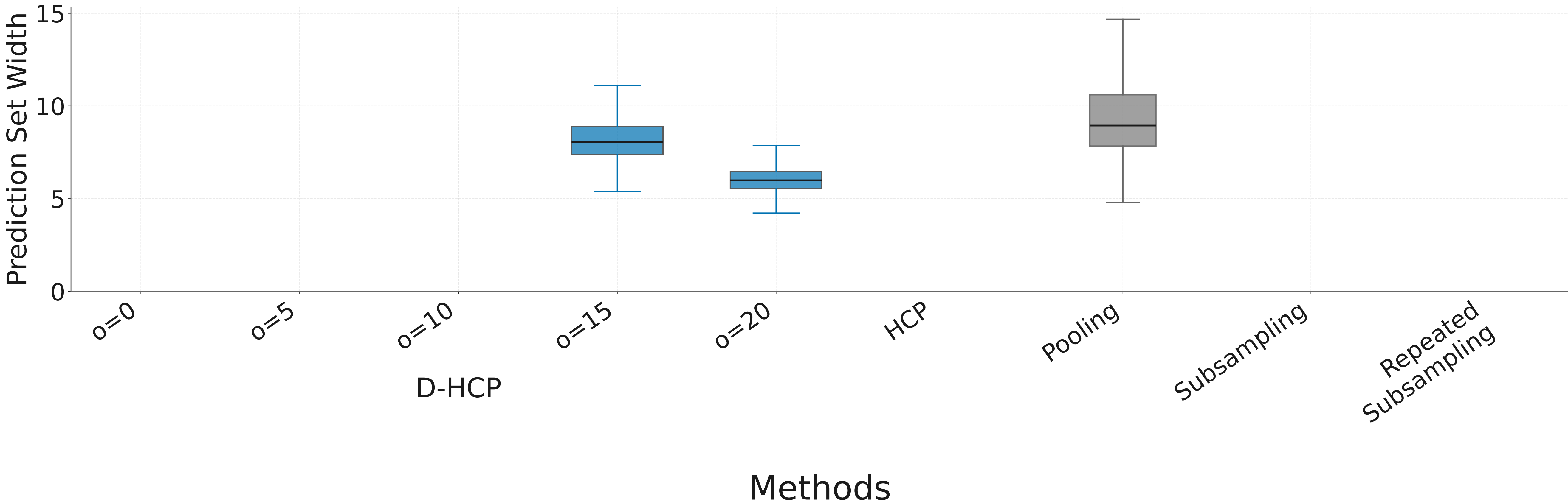
Fixed N_k = 21 : Prediction set width (all methods)
