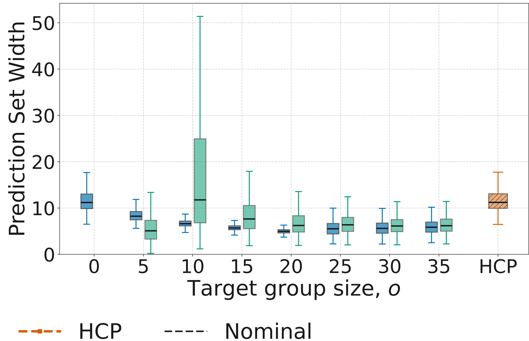
Prediction Set Width
