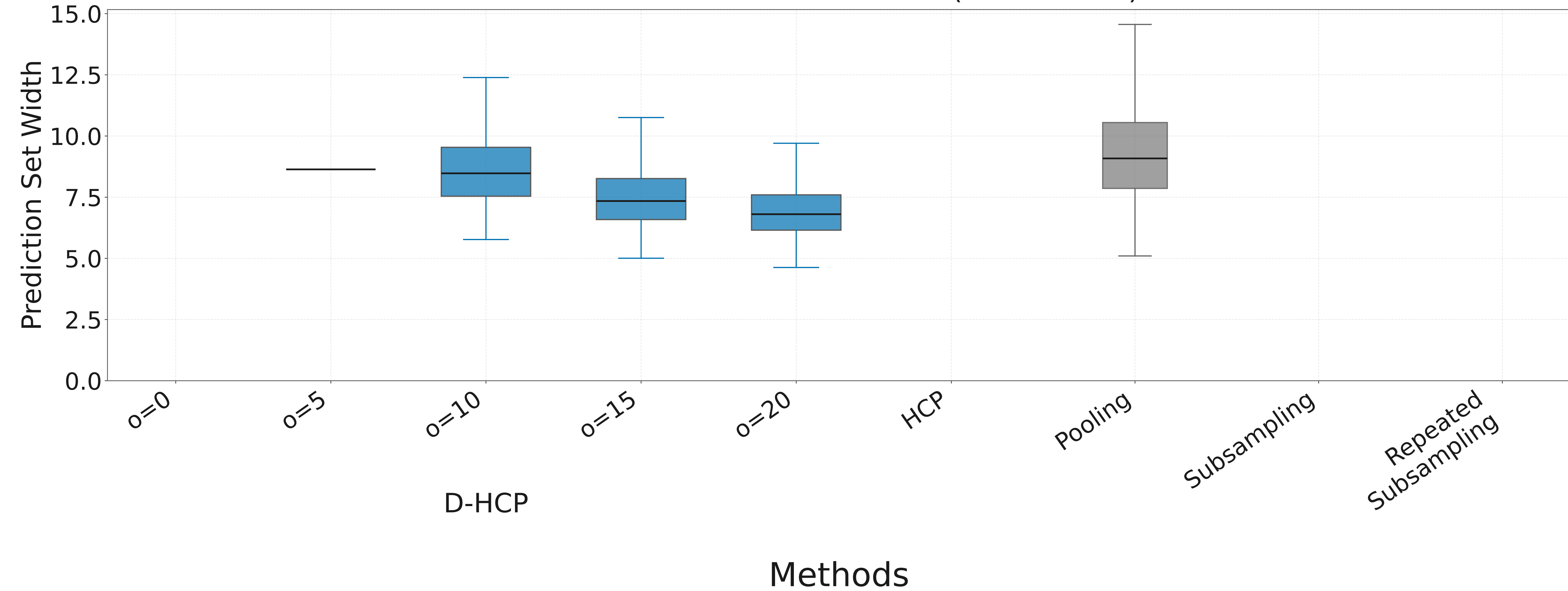
Poisson: Prediction set width (all methods)
