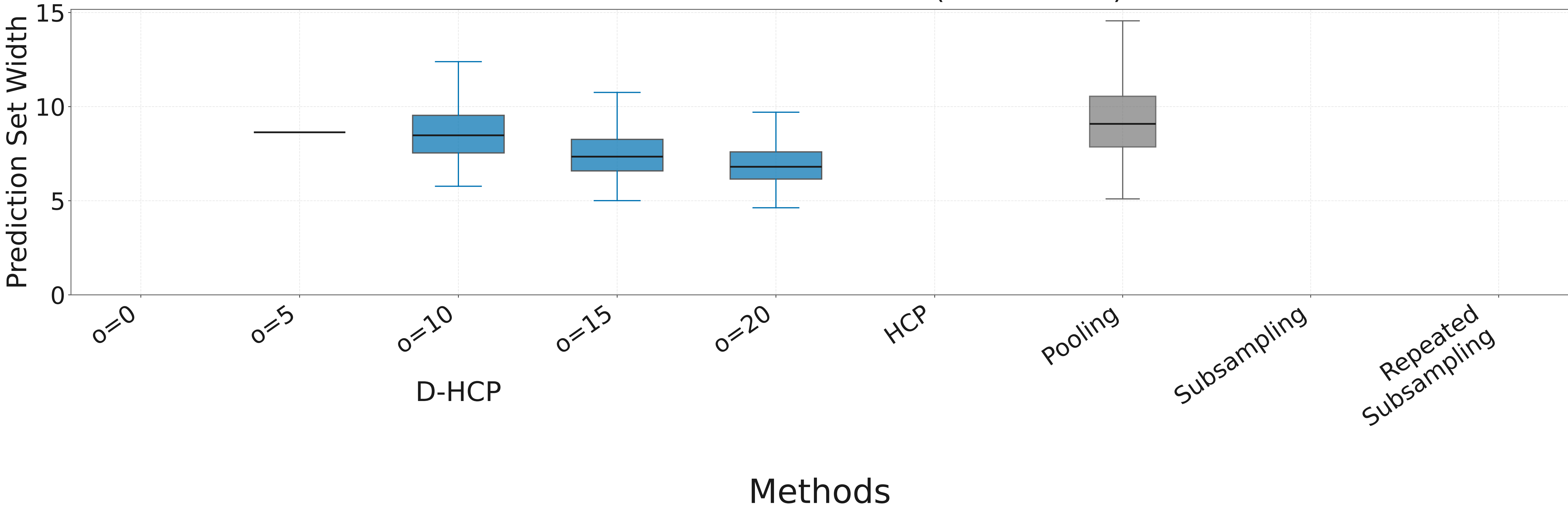
Poisson: Prediction set width (all methods)
