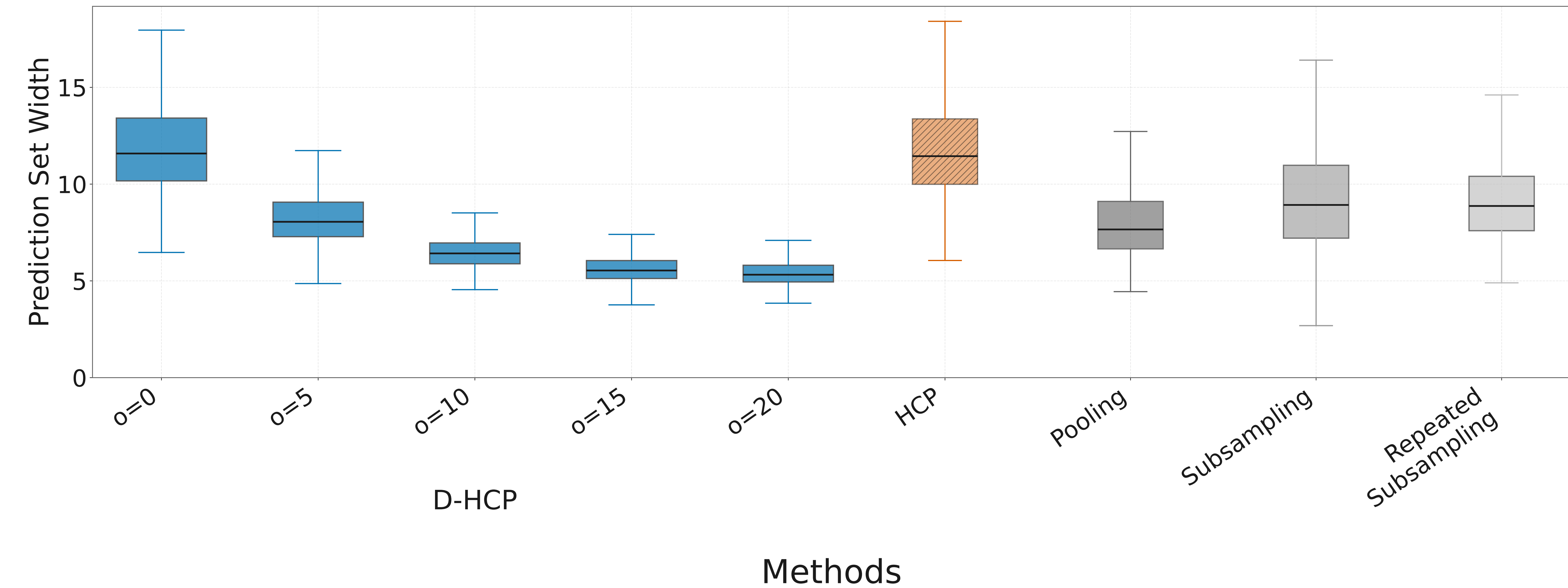
Poisson: Prediction set width (all methods)
