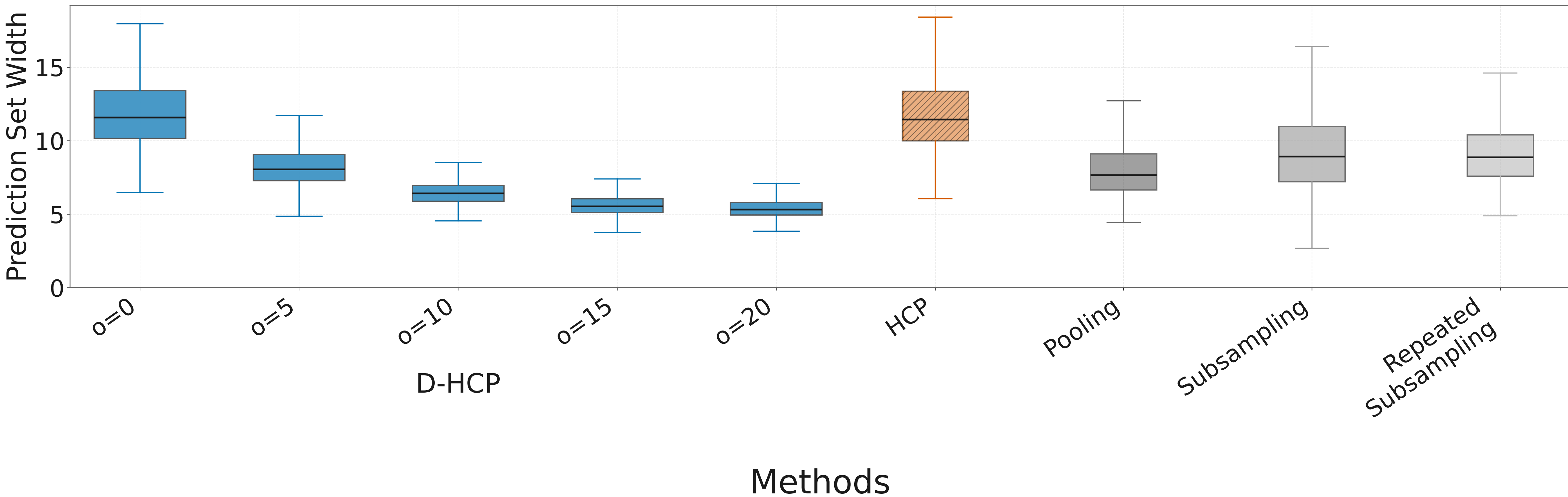
Poisson: Prediction set width (all methods)
