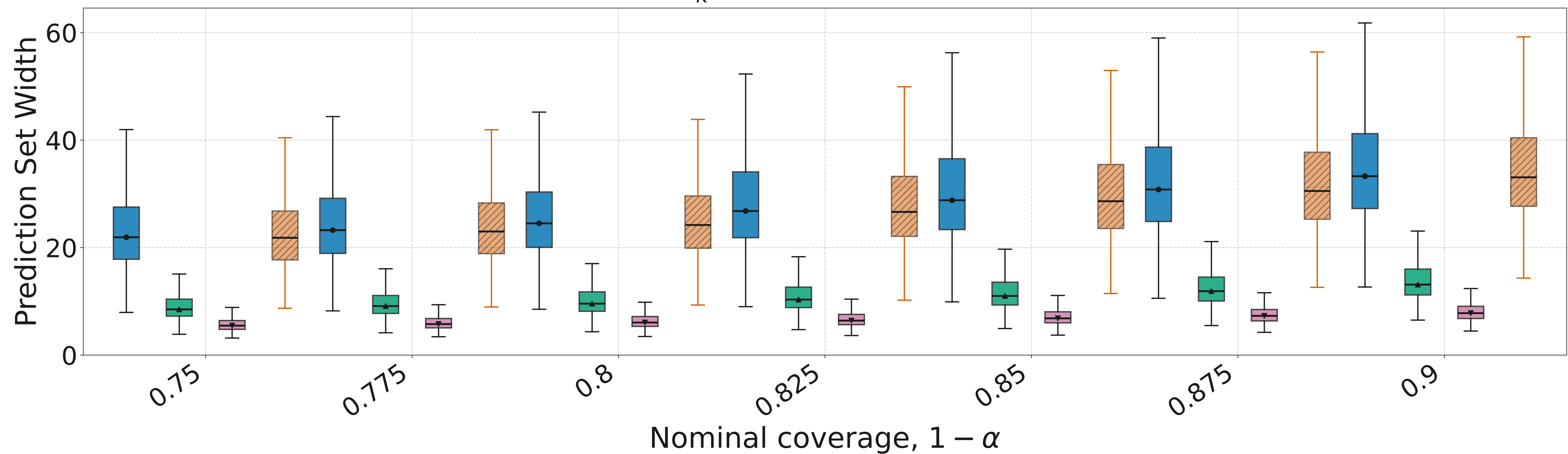
Fixed N_k = 21 : widths over 1 - \alpha
