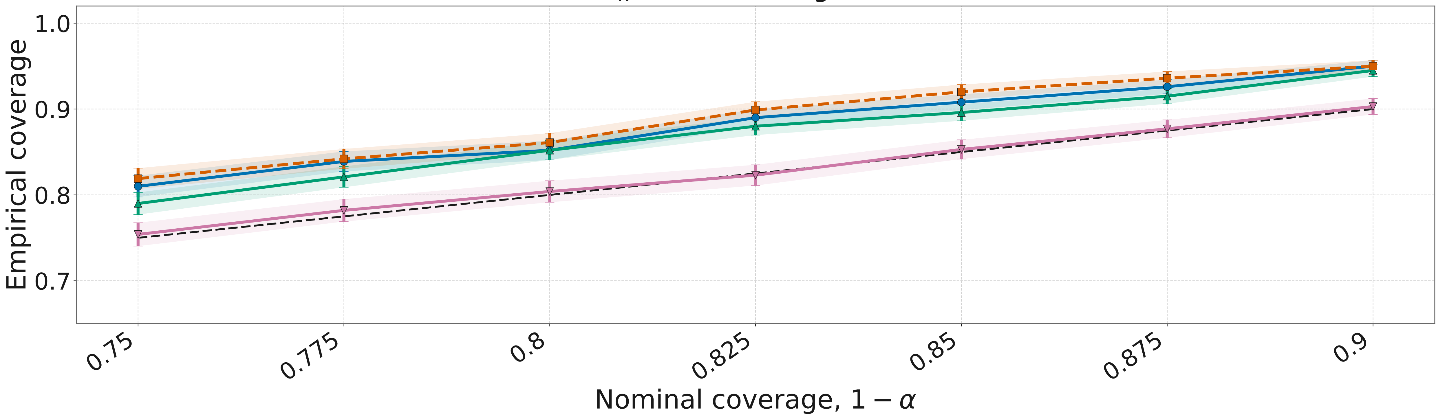
Fixed N_k = 21 : coverage over 1 - \alpha
