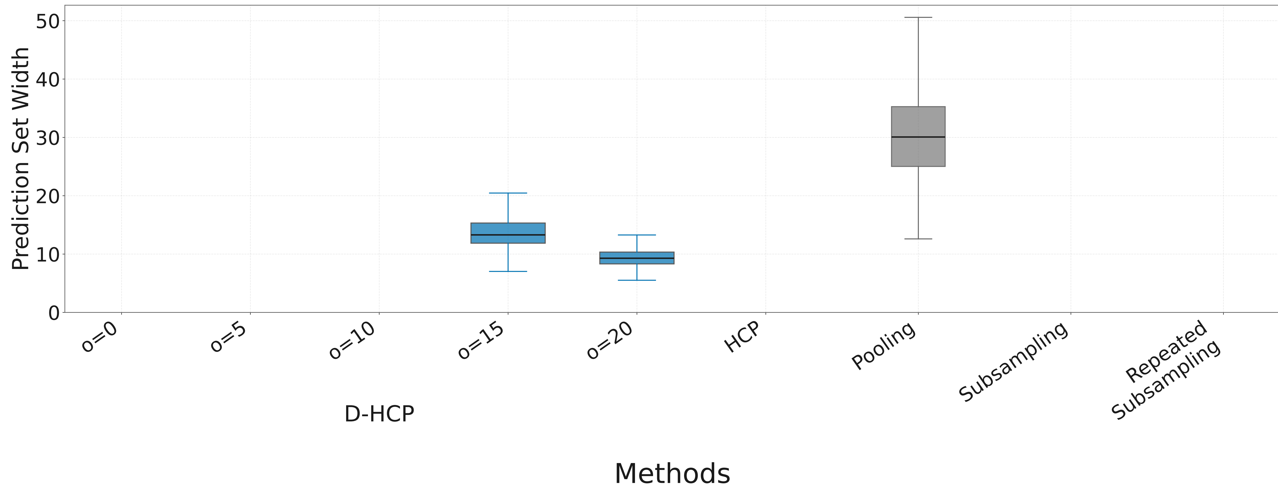
Fixed N_k = 21 (RF): Prediction set width (all methods)
