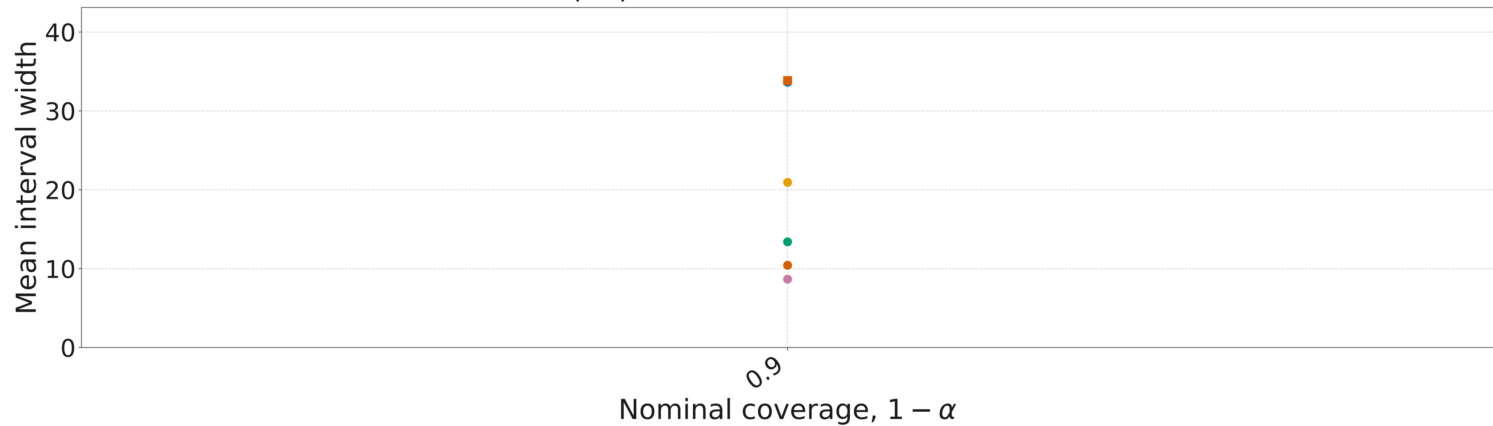
Poisson (RF): Width with standard-error bands
